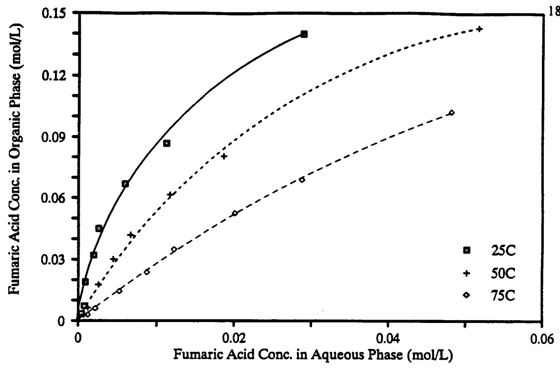
Figure A.7 Fumaric acid distribution into 0.064M Alamine 336 and MIBK at three temperatures.
