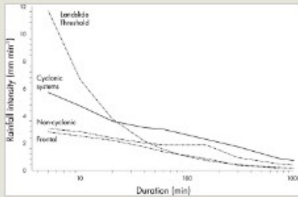
Figure 4.6 Rainfall intensity-duration curves by Caribbean storm type and a landslide rainfall intensity-duration threshold curve for Puerto Rico. (From Scatena et al. 2005.)
