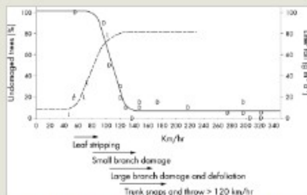
Figure 4.8 Maximum wind gusts versus percent of tree damage (D) and amount of litterfall (L) for the Luquillo Mountains. The types of canopy damage commonly observed for a given range of wind gusts are depicted by the arrows below the diagram. (After Scatena et al. 2005.)
