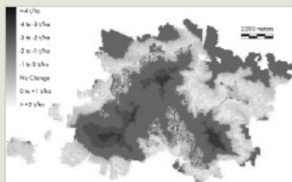
Figure 4.13 Simulated changes in soil organic carbon in response to an increase in temperature.
