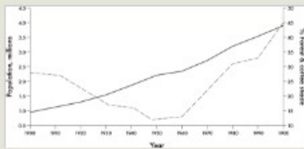
Figure 4.5 Island-wide population and forest cover (dashed line) by decade from 1900 to 2000.
