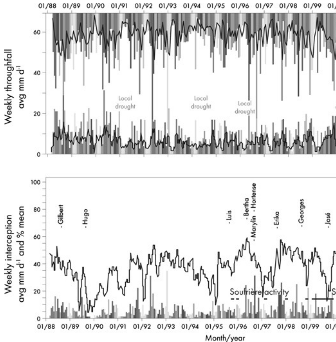
Figure 4.2 Weekly rainfall and throughfall and significant climatic events in the Bisley Research Watersheds, 1988 to 2003.
