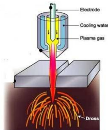
Figure 4.11: Schematic of plasma arc cutting process (TWI, 2012)
