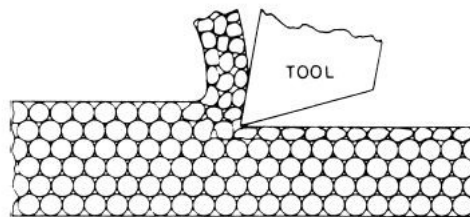
Figure 3.5: Deformation in the chip and workpiece resulting from machining (Kazanas & Lerwick, 2002)
