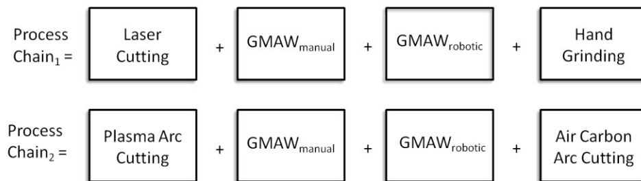
Figure 5.9: Process chain comparison
