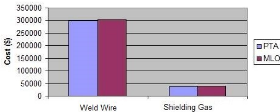
Figure 6.9: Comparison of Process Trade-off Analysis tool and Manufacturing Line Optimization results
