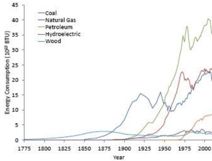
Figure 1.2: Historical energy consumption in the United States from 1775 – 2009 divided into each energy source (adapted from (U.S. Energy Information Administration, 2012)).
