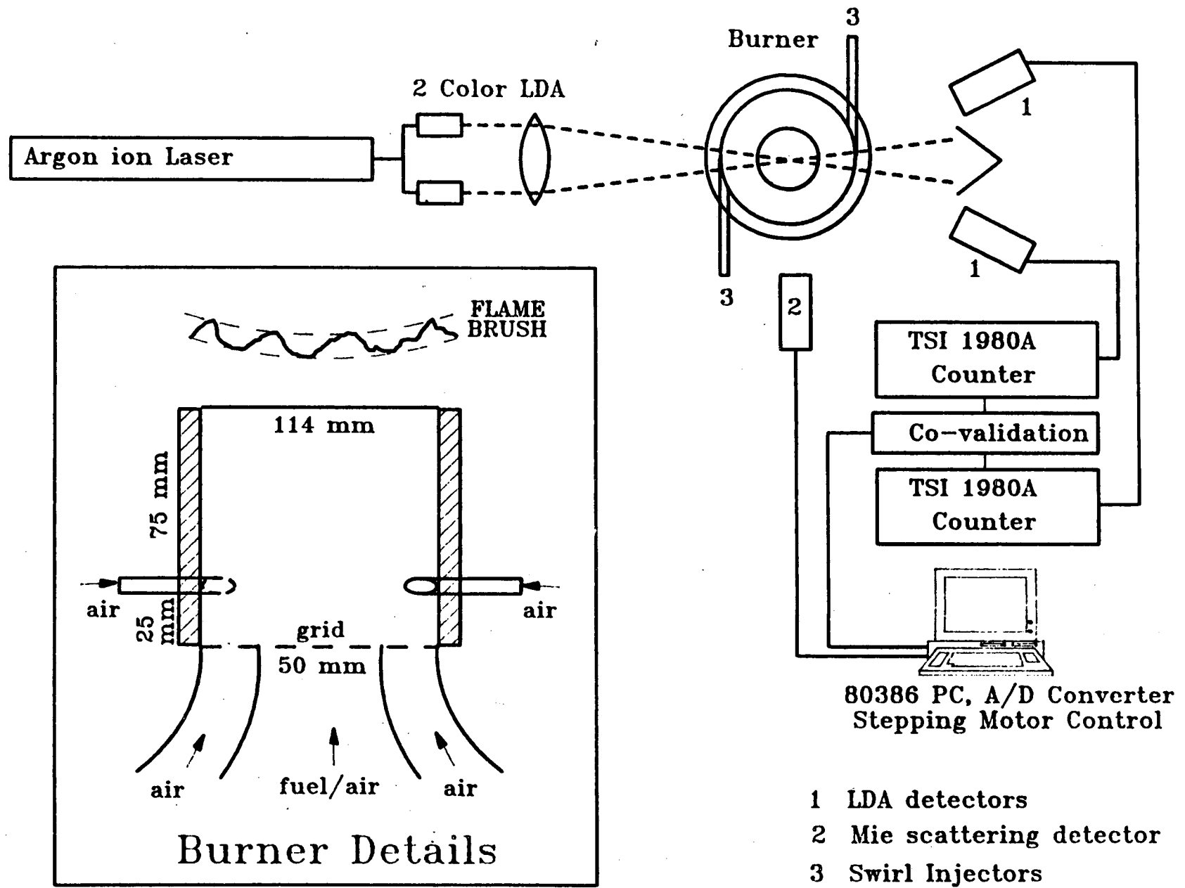
Fig. 2 Schematics of the experimental and diagnostics systems.
