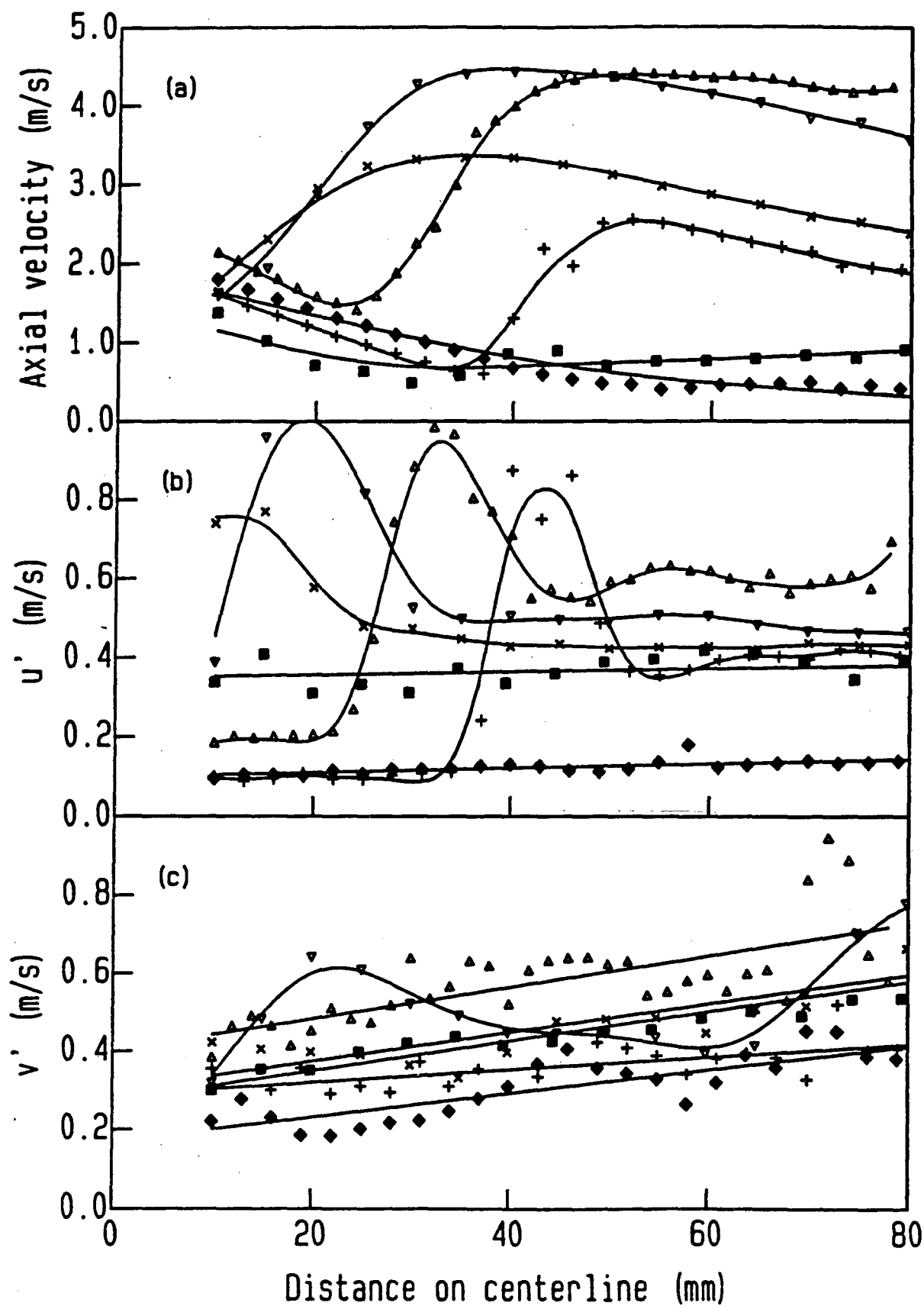
Fig. 4 Centerline mean and rms velocity profiles.
