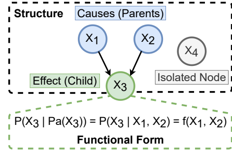
Figure 1: Causal graph. The edges (arrows) define the causal structure : For a given edge, the source node is the “parent” (cause) and the destination node is the “child” (effect). Isolated nodes are not involved in any causal relationships. The child node X_3 has a conditional probability P defined by the functional form (one type of overhypothesis) of the relationship with its parents Pa(X_3) .
