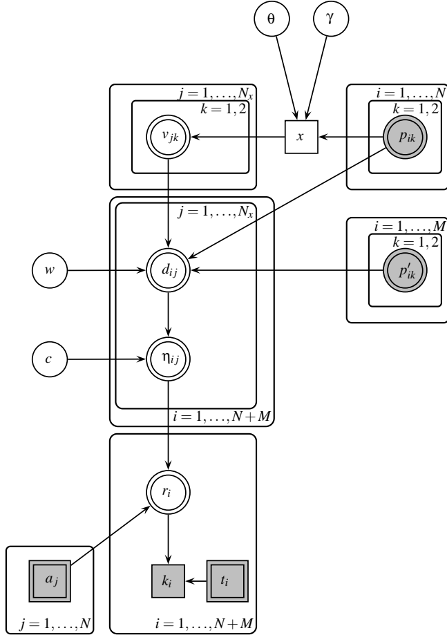
Figure 2: Graphical model representation of the hierarchical VAM used in the applications.
