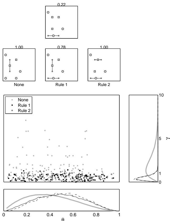
Figure 6: Hierarchical VAM account of the Nosofsky et al. (1989) category data.
