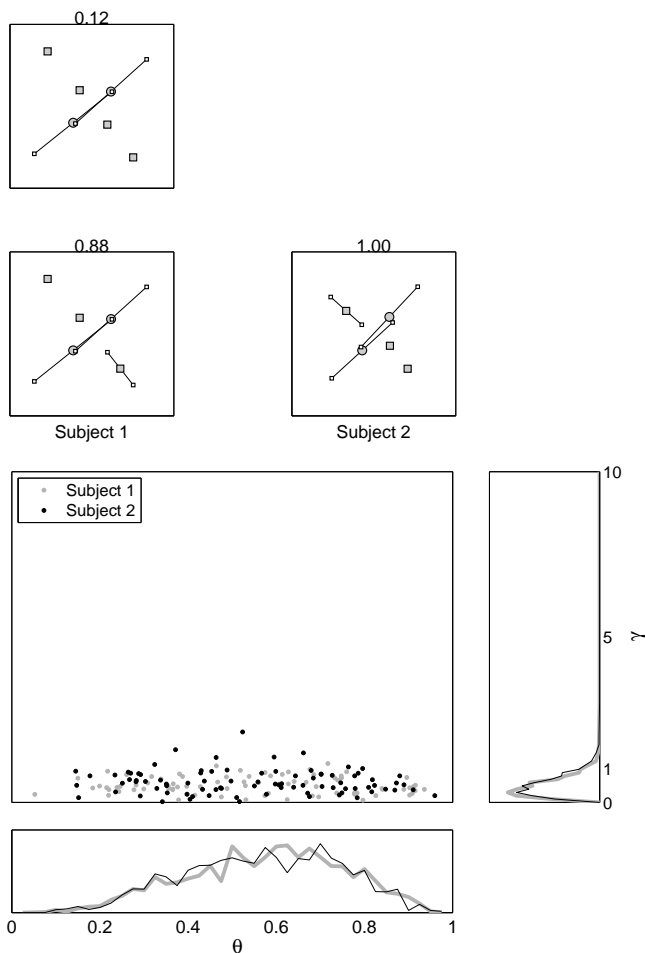
Figure 5: Hierarchical VAM account of the Nosofsky (1986) Criss-Cross category data..
