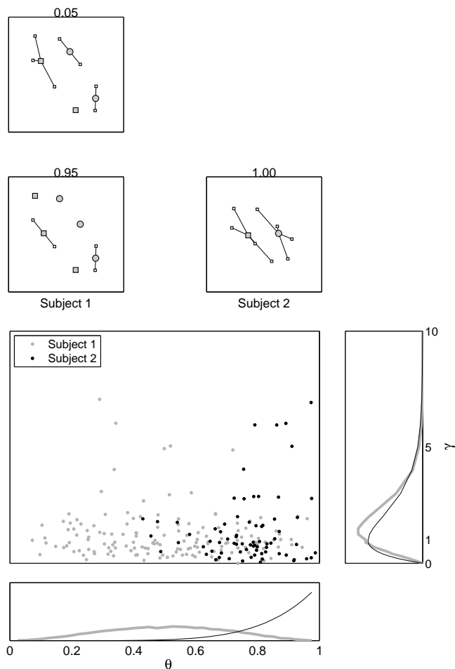
Figure 4: Hierarchical VAM account of the Nosofsky (1986) Diagonal category data.
