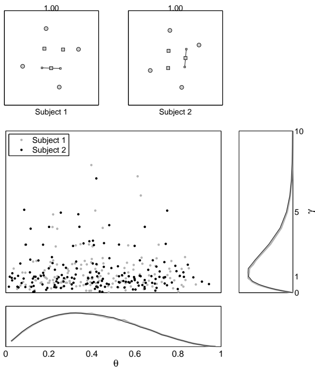
Figure 3: Hierarchical VAM account of the Nosofsky (1986) Interior-Exterior category data.
