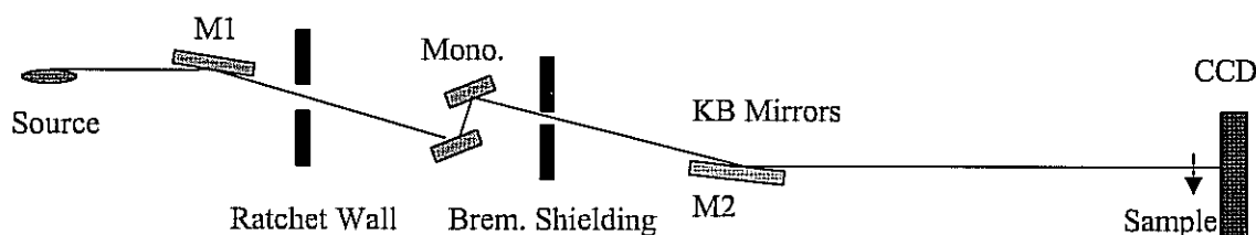
Figure 2: Beamline layout for the two experimental stations described in the text.
