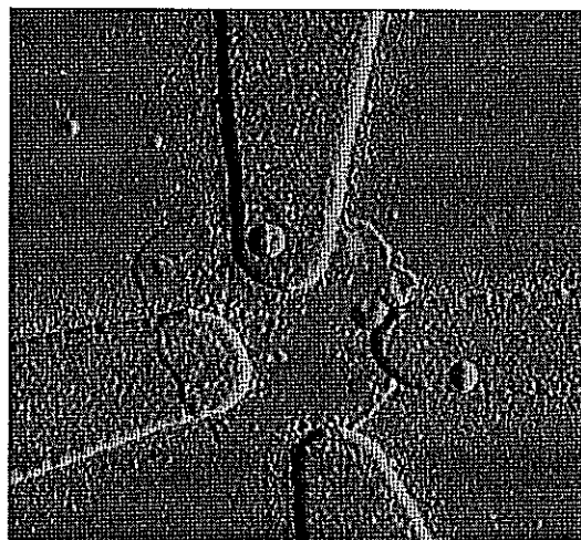
Figure 5: Submicron graphene platelet with attached electrodes.
