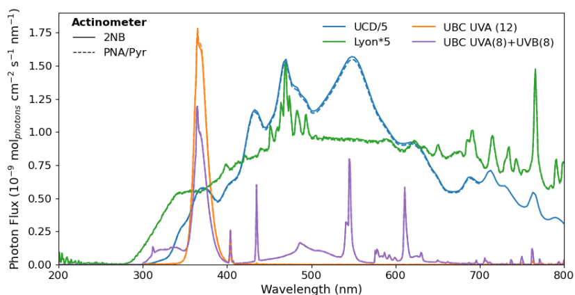
Figure S11. Photon flux calibrated using the 2NB chemical actinometer (solid line) and PNA/Pyr actinometer (dashed line) for experimental set ups used in this study. UCD photon flux is reduced by a factor of 5x and Lyon photon flux is increased by a factor of 5x for a clear comparison of all experimental set ups
