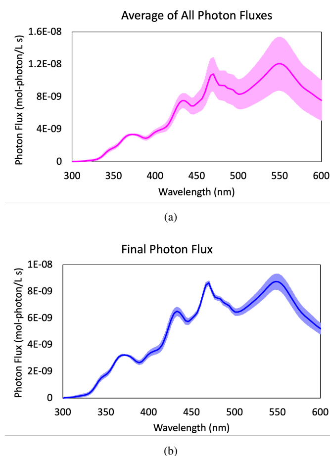
Figure S21. Showing a) Average and standard deviation of 60 photon flux measurements of the UCD simulated sunlight. b) Average and standard deviation of UCD photon flux in best agreement with the singlet oxygen quantum yield of perinaphthene.
