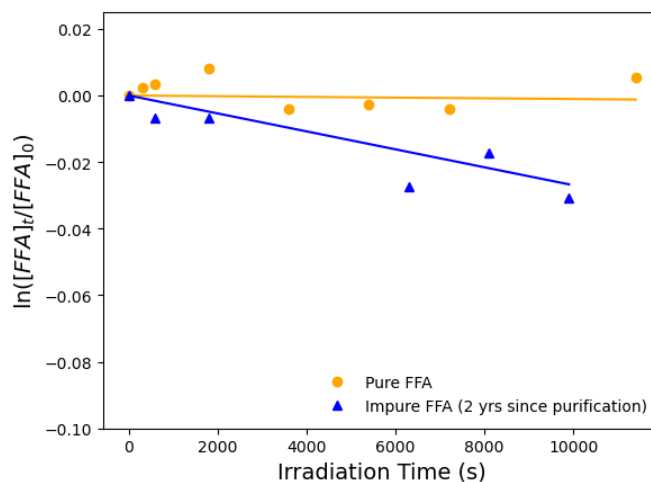
Figure S13. Direct photodegradation of furfuryl alcohol (FFA) using the UBC UVA set up, showing FFA that has not been purified for 2 years in blue and purified FFA in orange.
