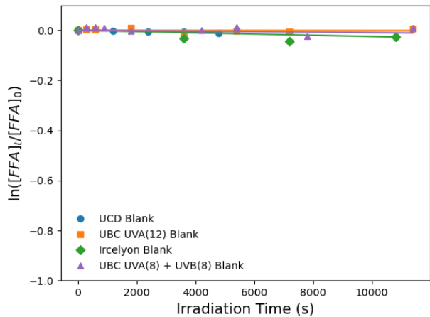
Figure S1. Blank FFA control experiment for each research group. Blank controls are prepared the same as experimental solutions, and are irradiated for the same amount of time as experimental solutions, however a sensitizer is not added.
