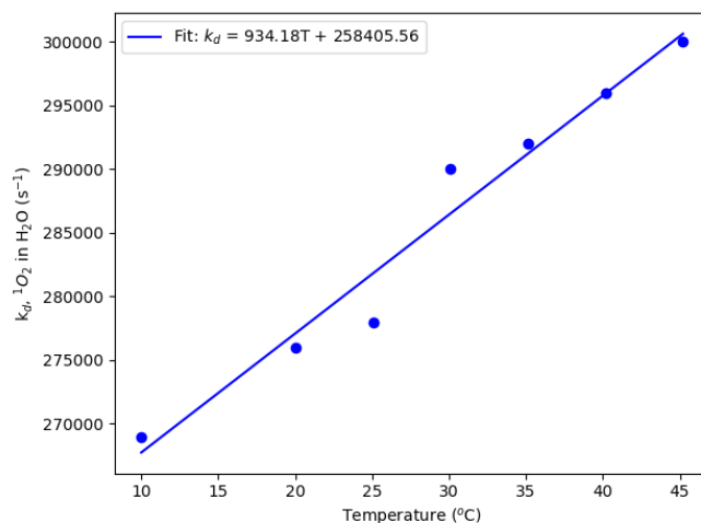
Figure S18. Temperature dependence of the deactivation of ^1O_2^* in water from Appiani et al. (2017).
