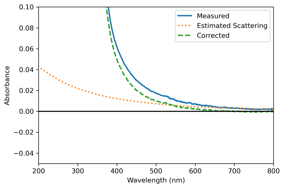
Figure S16. Measured lignin absorbance (20 mg/L), estimated scattering and a corrected absorbance spectra. A particle concentration of 1.18 \times 10^{13} \text{ m}^{-3} and a mean particle diameter of 142 nm is used based on previous measurements.
