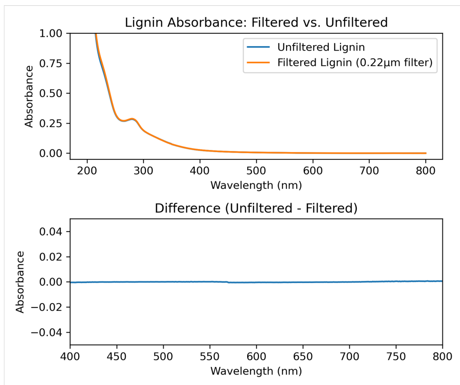
Figure S15. Absorbance of lignin before and after filtering with a 0.22μm filtering. Showing raw absorbance of unfiltered and filtered samples on the top panel and the difference (unfiltered-filtered) in the bottom panel.
