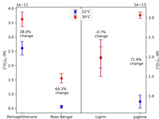
Figure S19. Temperature dependence of ^1O_2^* steady state concentrations produced from photosensitizers: perinaphthenone, Rose Bengal, lignin, and juglone, using temperature corrected rate constants.
