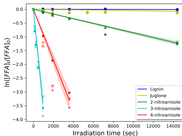
Figure S14. FFA decay of lignin and juglone, along with three nitroanisole compounds (atmospherically relevant molecules, not studied in depth here) during irradiation in the absence of O_2 (purged with N_2 ). Different symbols represent triplicate measurements, and the shaded area represents standard deviation from the mean linear fit.
