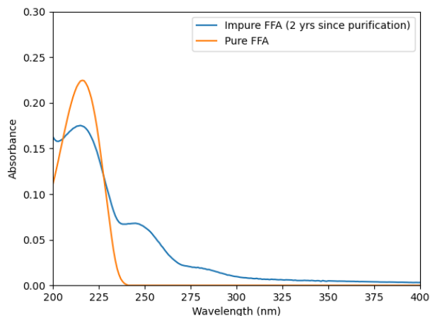
Figure S12. Absorbance of furfuryl alcohol (FFA) at UBC, showing FFA that has not been purified for 2 years in blue and purified FFA in orange.
