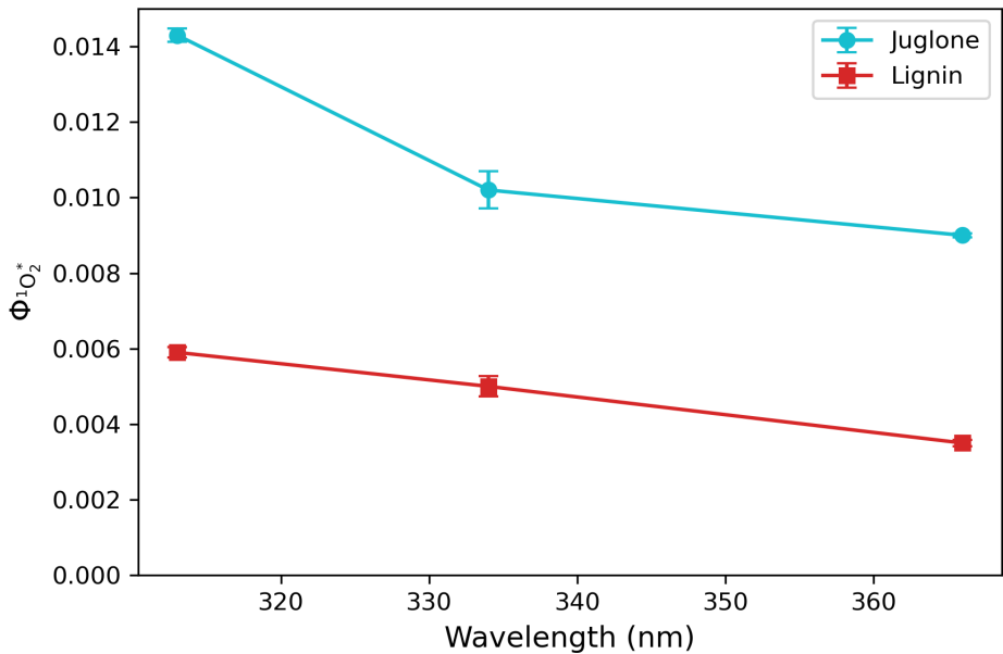
Figure S20. Quantum yield dependence on wavelength for lignin and juglone sensitizers. Experiments conducted at UCD, described in section 2.8.
