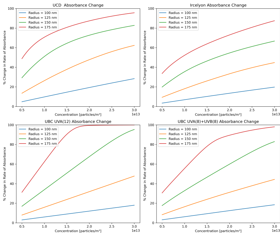
Figure S17. Sensitivity analysis of the impact of particle scattering on the rate of light absorbance. The percentage change is calculated as \left( \frac{R_{\text{abs, No scat}} - R_{\text{abs, scat}}}{R_{\text{abs, No scat}}} \right) \times 100\% . Note that % change values are shown as positive values, but scattering results in a decrease in light absorbance
