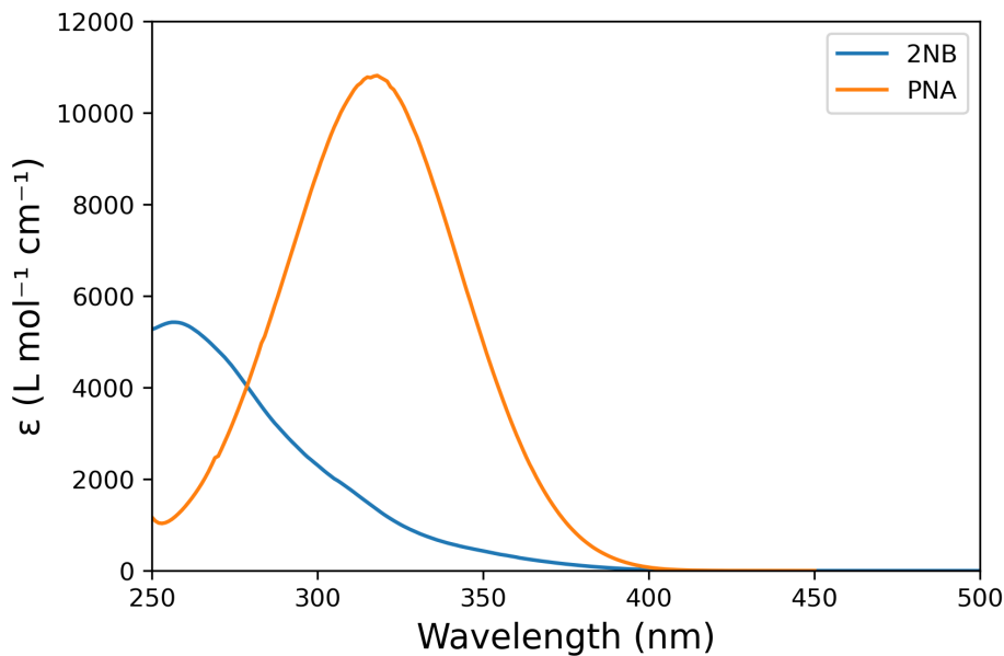
Figure S10. Molar absorptivity of p-nitroanisole (PNA) and 2-nitrobenzaldehyde (2NB) from 250 – 500 nm.
