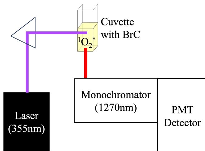
Figure S8. Schematic diagram of a time resolved phosphorescence laser spectroscopy experimental set up for ^1\text{O}_2^* detection.
