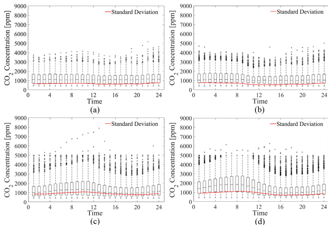
Fig. 6. Hourly averaged CO 2 concentrations in dormitory rooms during: (a) weekdays in the HVB; (b) weekends in the HVB; (c) weekdays in the LVB; and (d) weekends in the LVB.
