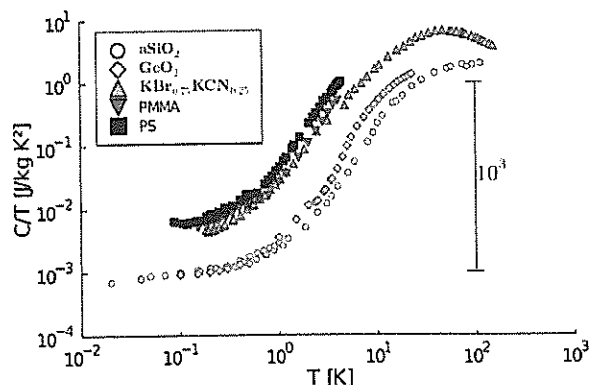
Fig. 1. C/T vs. T for amorphous \text{SiO}_2 (aSiO 2 ) [3, 4], \text{GeO}_2 [3, 5], \text{KBr}_{0.75}\text{CN}_{0.25} [6], PMMA [7–9], and PS [8, 9] shows a steep rise by two to three orders of magnitude between 3–10 K.
