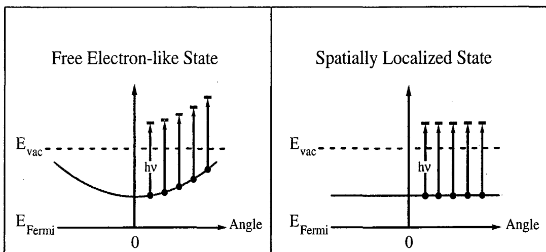
Figure 2.5: Schematic diagram of angle resolved two photon photoemission. For an electron to be detected when \theta > 0 , the electron must have a component of momentum parallel to the surface, p_{||} = \hbar k_{||} . As \theta increases, so does p_{||} . By measuring the parallel dispersion, the p_{||} dependence of the photoelectron kinetic energy, the interfacial band structure can be determined. The quantum number k_{||} characterizes nearly free electronic bands. For nearly free electron bands, p_{||} determines the energy and the dispersion will be parabolic. These states with well defined momenta are spatially delocalized, in accordance with the Heisenberg uncertainty principle. For spatially localized electronic states, k_{||} will not be a good quantum number, and the energy will no longer depend on p_{||} . Such states will have flat dispersions.
