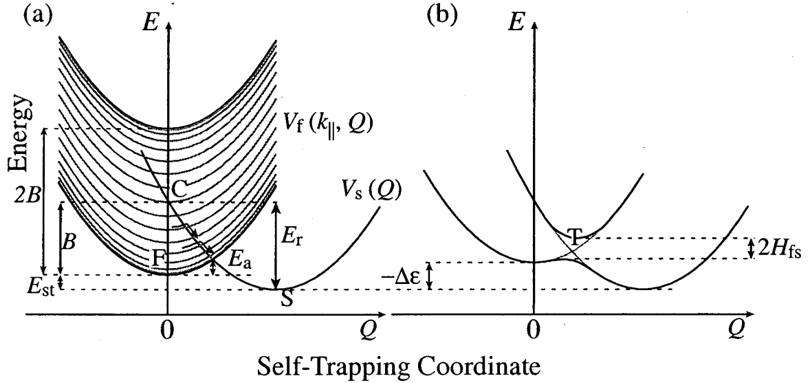
Figure 5.7: (a) Schematic representation of electron localization. Curves V_f(k_{\parallel}, Q) and V_s(Q) correspond to the delocalized and localized states, respectively. Each V_f(k_{\parallel}, Q) corresponds to a different k_{\parallel} state with a band energy of E_{\parallel} . For definitions of the other parameters, see the text. (b) A schematic representation of the influence of electronic state coupling ( H_{fs} ) in electron localization. For large H_{fs} , the electron adiabatically follows the lowest energy curve, while for small H_{fs} only a fraction of the electrons that reach the transition state transfer from the delocalized donor to the localized acceptor state.
