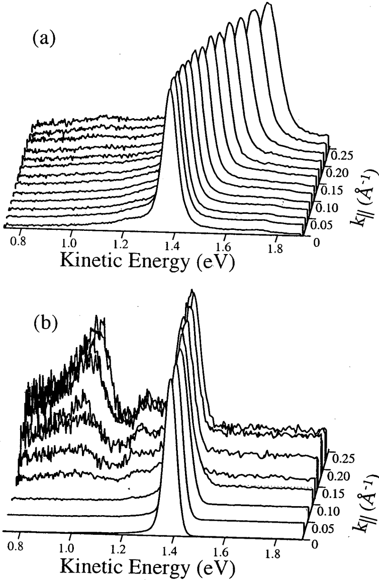
Figure 5.5: Femtosecond angle resolved kinetic energy spectra for a bilayer of anthracene adsorbed on Ag(111). (a) Plot of energy versus k_{||} for zero pump-probe time delay. The dispersive n = 1 dominates the spectra. (b) Plot of the energy versus k_{||} for a one picosecond pump-probe delay. Non-dispersive features dominate the spectra, with three peaks clearly present at higher k_{||} . All spectra are normalized to the highest intensity peak in each spectrum. The absolute amplitude of the highest energy non-dispersive feature decreases with increasing k_{||} , while the other two non-dispersive features have amplitudes that increase with increasing k_{||} .
