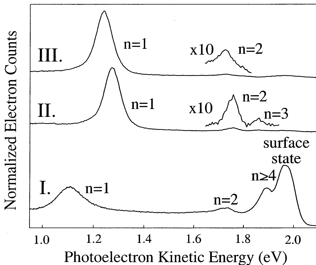
Figure 4.2: Photoelectron kinetic energy spectra for a monolayer I., a bilayer II., and a trilayer III. of benzene adsorbed on Ag(111). Variations in the photoelectron kinetic energy reflect variations in wavelength, workfunction, and binding energy. The persistence of the occupied surface state for the monolayer coverage results in the resonant excitation of n \geq 4 with 3.9 eV photons. Image state binding energies are reported in Table 4.2.
