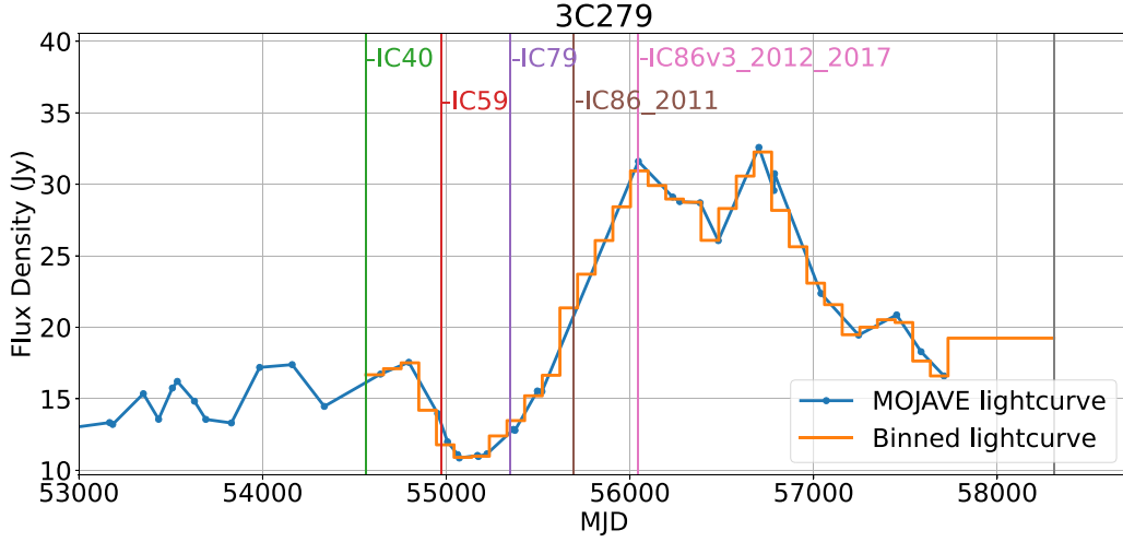
Figure 2. Example binned light curve (orange line) using MOJAVE data (blue data points) for one source (3C279) along with different IceCube data sets, and their time coverage is shown with the corresponding data set name. The light curve is binned using equal time binning within the 10 yr IceCube data shown here by the vertical lines. Left to right, the bins are shown as green to red (2008–2009; IC-40), red to purple (2009–2010; IC-59), purple to brown (2010–2011; IC-79), brown to pink (2011–2012; IC86_2011), and pink to gray (2012–2017; IC86v3_2012_2017).
