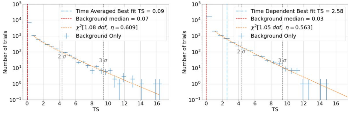
Figure 7. Background distribution plots derived for the time-averaged (left) and time-dependent (right) cases.
