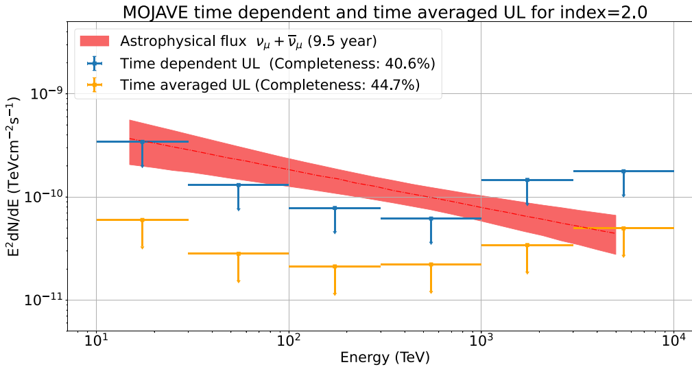
Figure 5. Differential upper limits (ULs), for an index of 2.0, derived from the time-dependent (blue) and time-averaged (orange) analyses in half-decade energy bins are shown here. The diffuse astrophysical muon neutrino flux measurements are taken from Abbasi et al. (2022a). Note that the upper limits shown here are differential and binned with energy, while the astrophysical flux is an energy-integrated measurement shown here only for reference.
