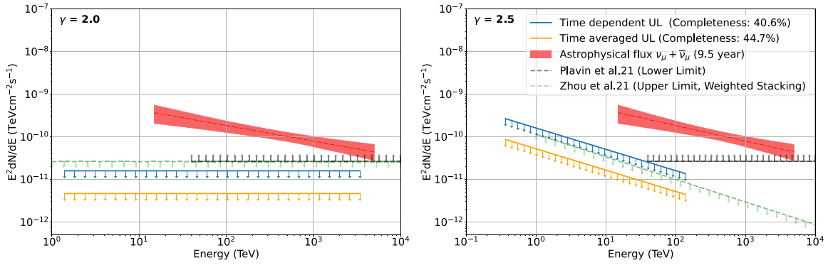
Figure 4. Upper limits (ULs) per neutrino ( \nu + \bar{\nu} ) flavor, for an index of 2.0 (left) and 2.5 (right solid line), derived from the time-dependent (blue) and time-averaged (orange solid line) analyses are shown here along with the lower limits (gray-dashed line) reported by Plavin et al. (2021). Note that while the samples and methodology used by Plavin et al. (2021); Zhou et al. (2021; green dashed line), and this work are different, making a 1:1 comparison difficult, they are shown here to highlight the differences in the results. The diffuse astrophysical muon neutrino flux measurements are taken from Abbasi et al. (2022a). The energy range of the upper limits shown for the time-averaged analyses reflects the region where 90% of detected signal neutrinos would fall. The energy range for the time-dependent scenario is kept similar to the time-averaged case.
