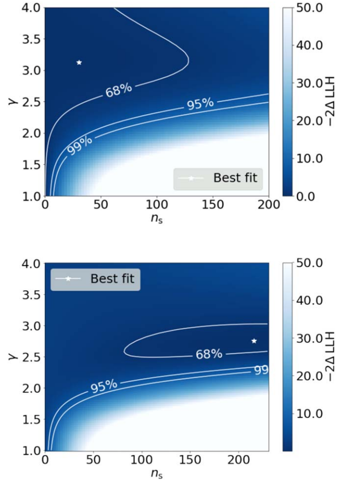
Figure 3. Likelihood maps for the n_s - \gamma values for the two analyses are shown here: time averaged (top) and time dependent (bottom). The plot also shows the 1\sigma , 2\sigma , and 3\sigma confidence intervals from the best fit, assuming Wilk's theorem with 2 degrees of freedom.
