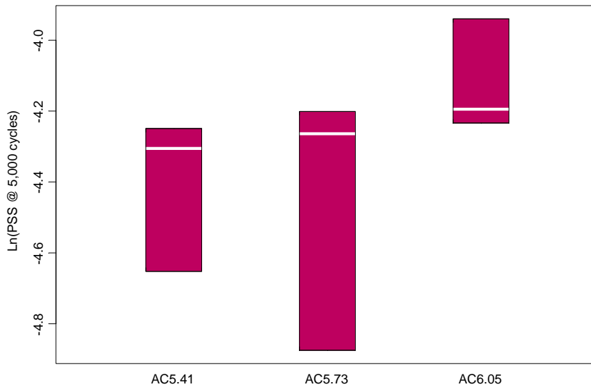
Figure A.2: Ln ( \gamma_p after 5,000 load repetitions) versus binder content, Weed PG 64-28PM, 15% RAP, 1.2% lime mix (50°C, 70 kPa stress).
