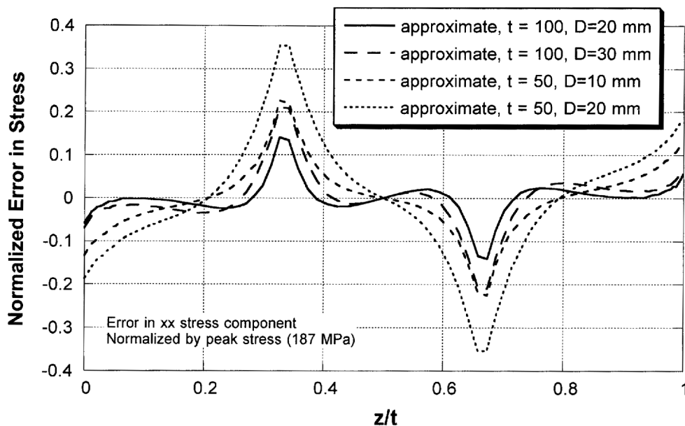
Fig. 9 Normalized error in residual stress in various DH geometries for approximate data reduction
