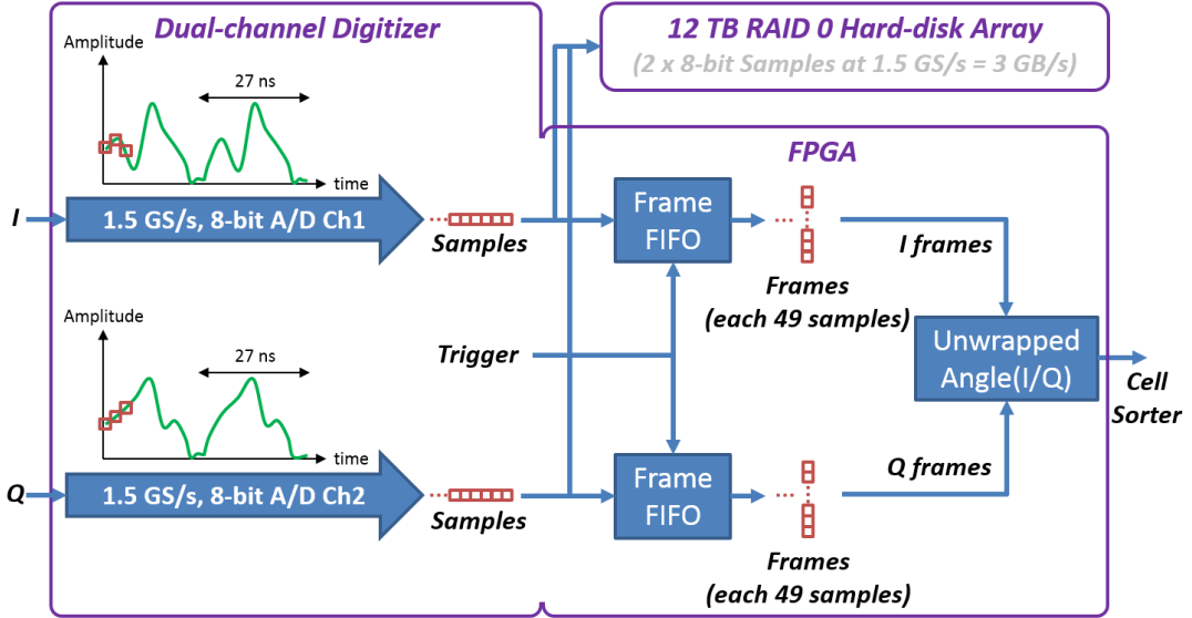
Figure 7.3: Digital signal processing system for acquisition of analog preprocessing unit outputs. This system is built with simple blocks such as argument calculator, unwrapper, and first in, first outs (FIFOs), which can be performed in real-time.
