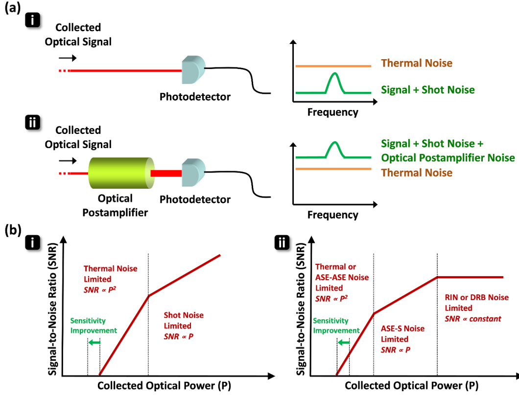
Figure 5.1: Detector sensitivity improvement by an optical postamplifier in high-speed detection. (a) (i) The optical signal is buried in the thermal noise of the photodetector (ii) whereas an optical postamplifier increases the optical signal with the thermal noise intact resulting in an improvement in the sensitivity of the detection system. (b) Comparison of the signal-to-noise ratios for photodetection (i) with and (ii) without an optical postamplifier shows that the optical postamplifier is useful when the detection sensitivity is thermal noise limited because the signal-to-noise ratio is directly proportional to the square of the collected optical power. Here, the signal-to-noise ratio and the collected optical power are both in logarithmic scale. ASE-ASE: amplified spontaneous emission self-beat; ASE-S: amplified spontaneous emission – signal beat; RIN: relative intensity noise; DRB: double Rayleigh backscattering. (These noise components are detailed in Section 5.3.).
