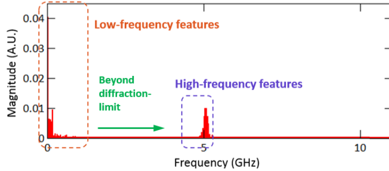
Figure 7.1: Spectral components of Coherent-STEAM signal. For a Coherent-STEAM setup with long enough arms' length mismatch the spectrum of the output signal shows two separate spectral bands. The low frequency components correspond to the intensity of the sample, while the high frequency components contain the phase information in addition to the intensity information of the cells.
