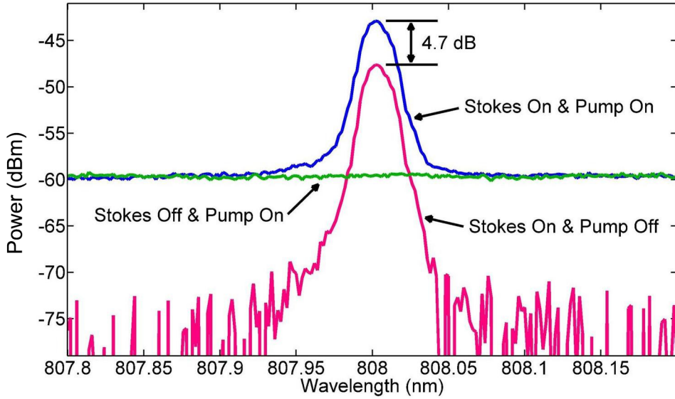
Figure 6.2: Experimental demonstration of Raman amplification at 808 nm in a single-mode fiber. The presence of the pump field amplified the Stokes field by 4.7 dB.
