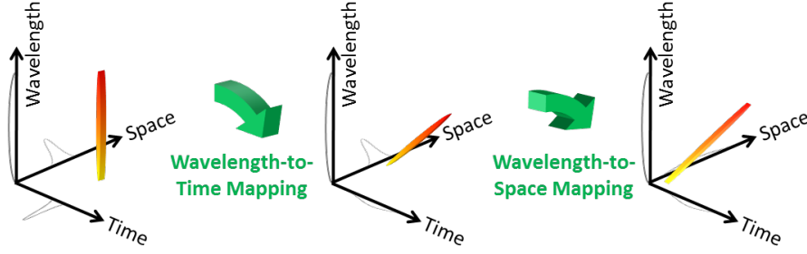
Figure 3.1: Concept of HDLS. HDLS operation relies on two high-speed mapping processes. First, the spectrum of each broadband optical pulse generated by a mode-locked laser is mapped to time. This wavelength-to-time mapping is performed by a temporal dispersive element such as a dispersive optical fiber or prism pair. Next, wavelength-to-space transformation is used to direct each wavelength component of the optical pulse to a unique point on the target. Overall, a one-to-one mapping between time and space is formed. Therefore, each point in HDLS field of view is sampled with an individual wavelength component of the optical pulse at a specific time. The repetition rate of the mode-locked laser determines the sampling rate of the HDLS.
