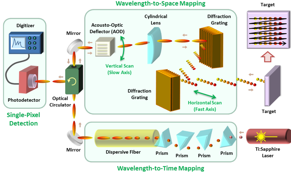
Figure 3.2: HDLS experimental setup. In a 2D demonstration of laser scanning with the HDLS, optical pulses generated by a mode-locked Ti:Sapphire laser with a center wavelength of 814 nm and a repetition rate of 90.8 MHz are dispersed in time using two pairs of prisms and a dispersive fiber. Pulses are deflected in the vertical direction using an acousto-optic deflector (AOD) at 105.4 kHz. Subsequently, the spectrum of each pulse is mapped onto a horizontal line using a pair of diffraction gratings. A combination of the vertical deflection and horizontal mapping leads to a 2D raster scan on the target. The pulse reflection off the surface of the target is converted via an optical circulator to an electrical signal using a single-pixel high-speed photodetector. This is possible due to the prior wavelength-to-time mapping, so that each wavelength component reaches the photodetector at a unique time, and the information of different points of the target are not overlapped. A 50 GS/s digitizer acquires the electrical signal from the photodetector, which corresponds to the spectrum of the optical pulses. After correction for the background envelope, the spectrum of each pulse reveals one horizontal line scan image of the target. Stacking up many of these line scans in accordance with the AOD scan frequency leads to a 2D raster scan of the target.
