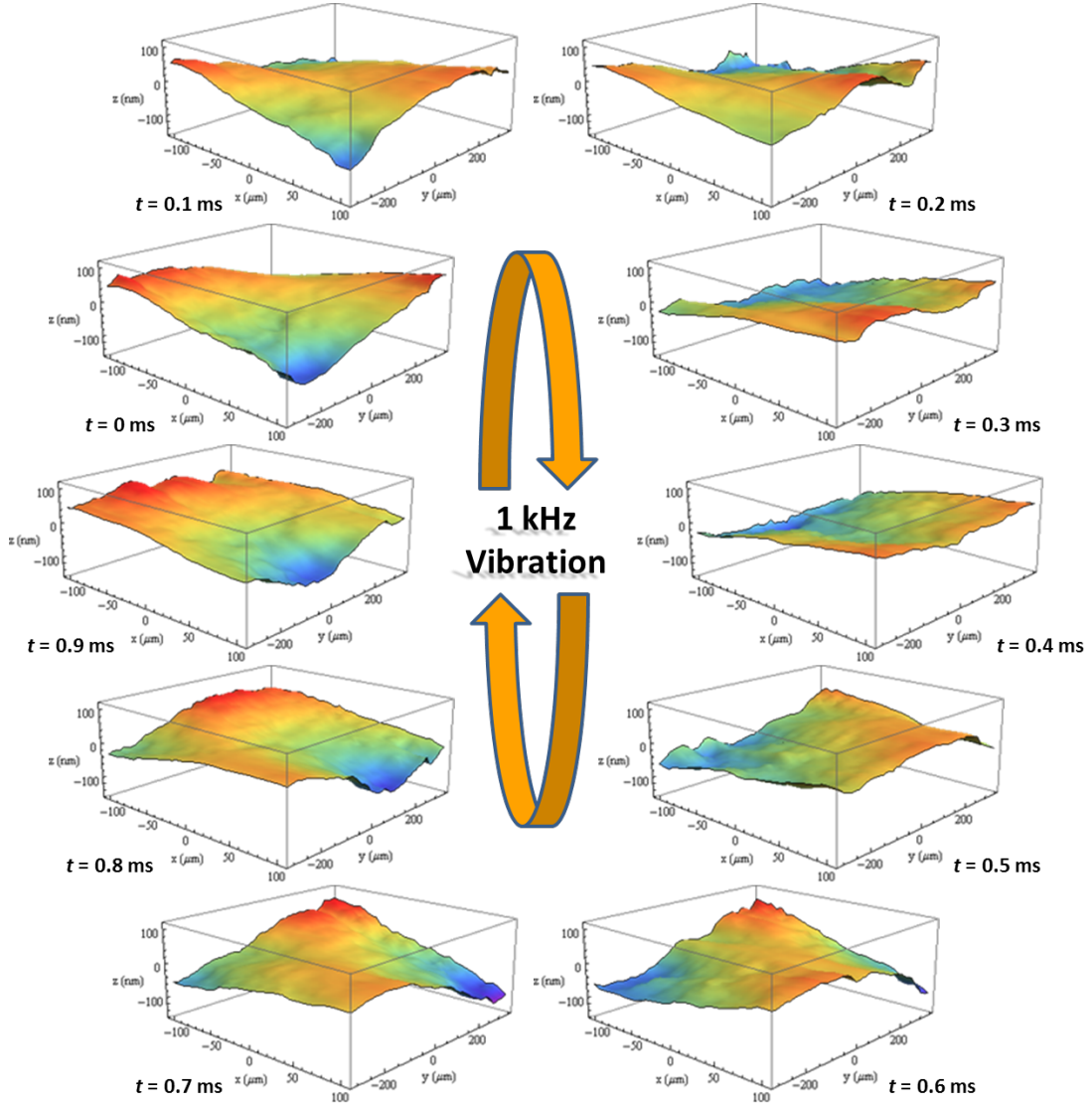
Figure 3.6: Surface vibration captured by the HDLS. Frames from 3D scans of a vibrating diaphragm by the HDLS show a period of nanomechanical vibrations at 1 kHz. Only one every ten scan is shown here.
