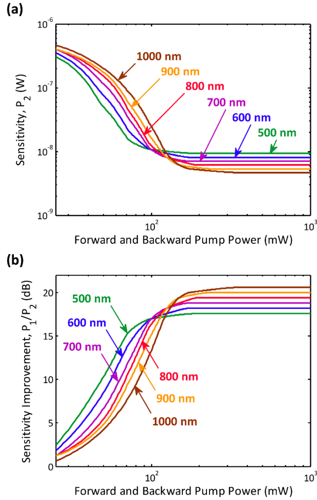
Figure 5.5: Predicted detection enhancement by optical postamplification over 100 MHz bandwidth in the visible to near-infrared spectral range. (a) Amplifier-enhanced sensitivity (minimum detectable power of the input signal) at various input wavelengths. (b) Sensitivity improvements by the postamplifier for a photodiode at various input wavelengths. Note that better sensitivities (lower minimum detectable powers) and higher sensitivity improvements are achievable at lower pump powers with the input signal at shorter wavelengths while better optimum sensitivities and sensitivity improvements can be obtained at longer input wavelengths.
