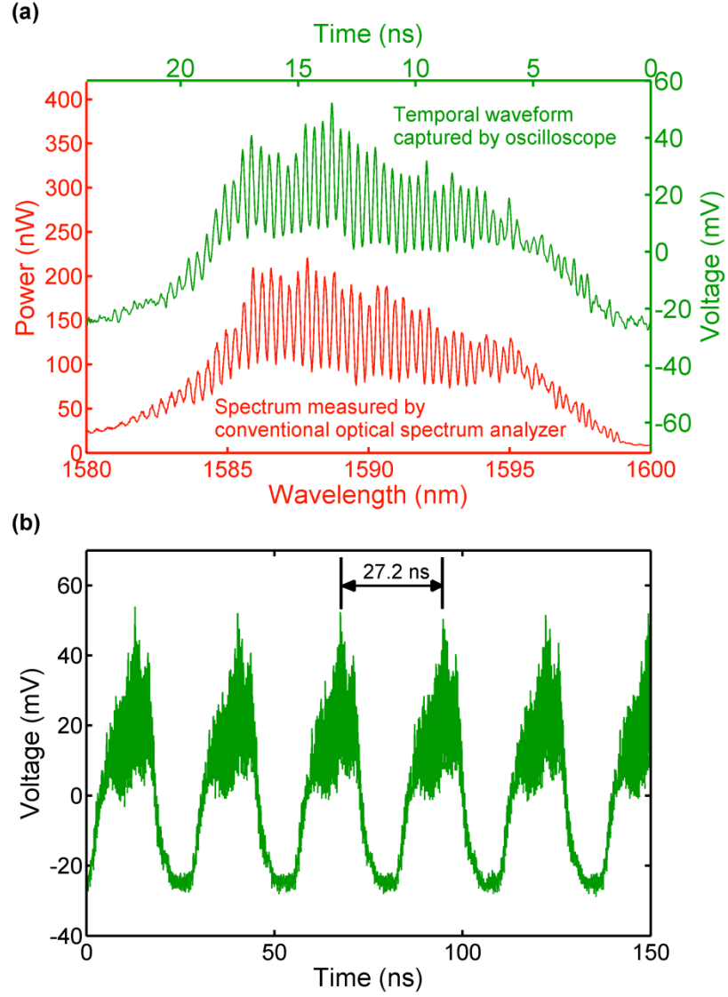
Figure 2.2: Basic performance of the STEAM vibrometer. (a) Temporal waveform of a single interfered pulse captured by the photodiode in comparison with the optical spectrum measured by a conventional optical spectrum analyzer. (b) Repetitive pulses (scans) with a time interval of 27.2 ns detected by the photodiode indicating that the STEAM vibrometer operates at 36.7 MHz scan rate.
