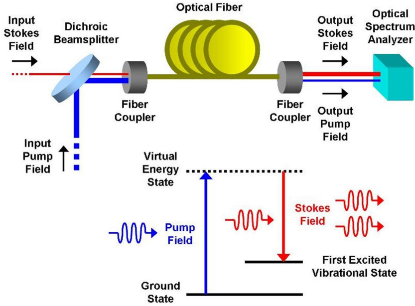
Figure 6.1: Distributed Raman amplification in a Ge-doped silica-core single-mode fiber. The input Stokes field is amplified by stimulated Raman scattering (SRS) in the fiber. The amplified Stokes field is detected by the optical spectrum analyzer.
