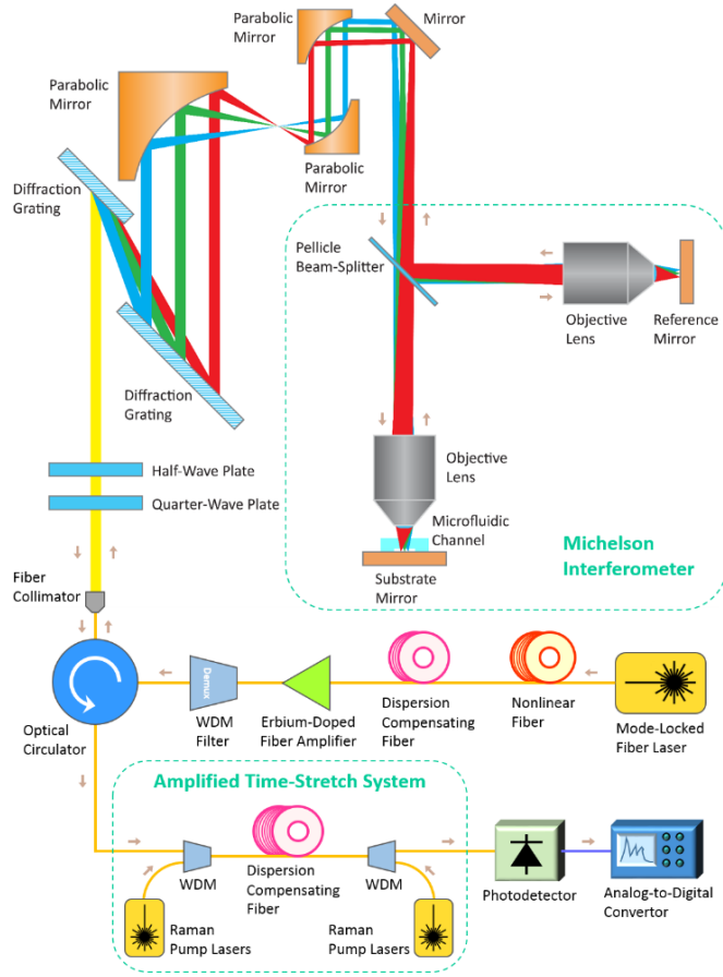
Figure 4.1: Optical setup of Coherent-STEAM. A Coherent-STEAM setup is formed by combination of STEAM and a Michelson interferometer. A pair of diffraction gratings generates a 1D rainbow with different wavelength components imaging different points on the cells flowing in a microfluidic channel. A pellicle beam-splitter and two identical long working-distance objective lenses are used to form the interferometer for phase measurement. Back apertures of objective lenses are fully illuminated with each wavelength component of the broadband mode-locked laser pulses to ensure diffraction-limited resolution. An amplified time-stretch system chirps, stretches, and amplifies each pulse, so that different wavelength components reach the photodetector serially. A very shallow microfluidic channel with hydrodynamic focusing is designed and fabricated to align cells within the focal depth of the system.
