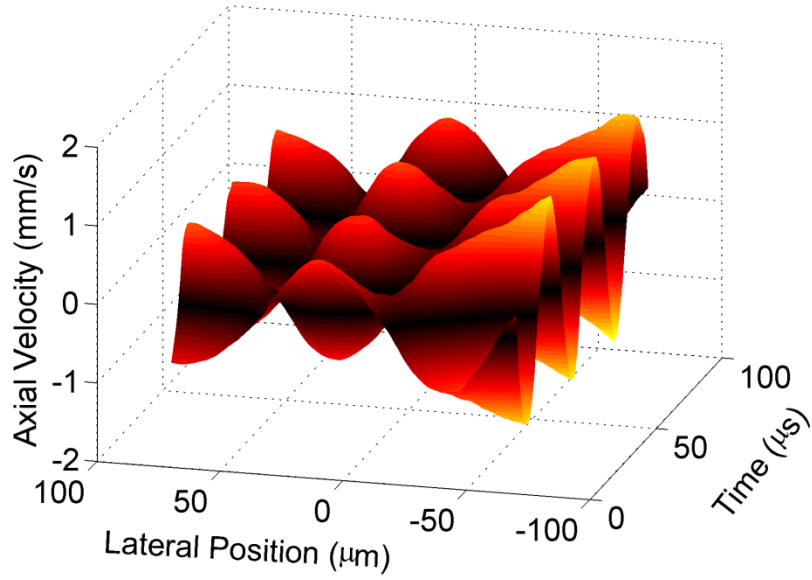
Figure 2.4: Axial velocity of the acoustic diaphragm obtained by the STEAM vibrometer. The diaphragm was driven to vibrate at 30 kHz (the same as in Figure 2.3).
