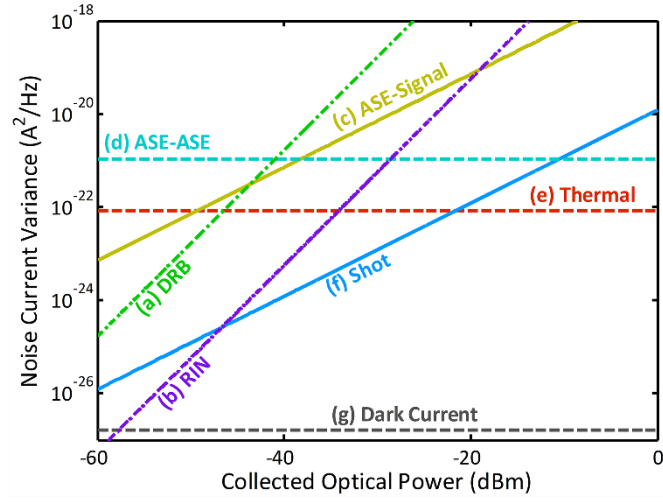
Figure 5.3: Noise photocurrent variance per 1 Hz detection bandwidth versus the input power to the optical postamplifier (collected optical power). (a) DRB noise, (b) pump-to-Stokes RIN transfer, (c) ASE-signal beat noise, (d) ASE-ASE beat noise, (e) thermal noise, (f) shot noise, and (g) dark current noise. The ASE-ASE beat noise and the thermal noise are dominant at low input powers while the RIN and DRB noise are significant at high input powers.
