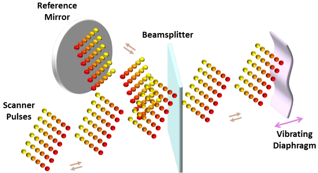
Figure 3.5: 3D surface profilometry or 2D surface vibrometry with the HDLS. 2D raster scans by the HDLS are used in conjunction with a Michelson interferometer to perform 2D surface vibrometry. A beamsplitter splits scan pulses into two arms. Optical pulses in one arm hit the target, and the light in the other arm (reference arm) is reflected intactly by a mirror. Reflected pulses from both arms are combined at the beamsplitter and form an interference pattern. If the reflectivity of the vibrating target is not changing rapidly, Hilbert transformation can be used to extract the relative optical phase of each wavelength component. Therefore, variations of the optical path length at each wavelength component are measured and used to form 3D surface profiles of the vibrating sample at a scan rate of 105.4 kHz with 0.4 nanometer axial resolution.
