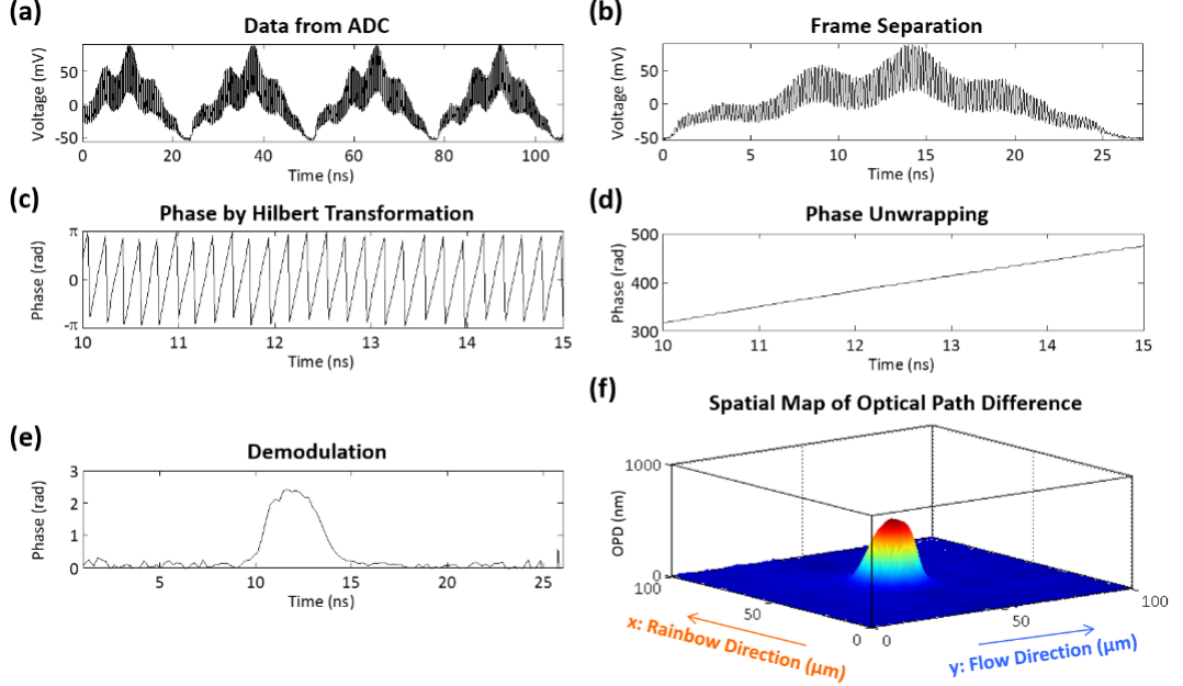
Figure 4.2: Digital signal processing of Coherent-STEAM. (a) The photodetector output signal is digitized and recorded by an ADC. This signal shows sequential laser pulses. (b) Each pulse is saved separately as a frame for further processing. (c) The analytic form of high-frequency components of each pulse is generated using Hilbert transformation, and the phase component of this analytic form is extracted. (d) An unwrapping algorithm is used to fix unrealistic phase jumps, and the result shows an approximately linear phase increase. (e) If the phase component of the interferometer fringe frequency is removed, the phase induced by cells in optical pulse can be seen. (f) Many of these line images generated from subsequent frames are used to form a spatial map of optical path difference in two dimensions, which is used for cell characterization.
