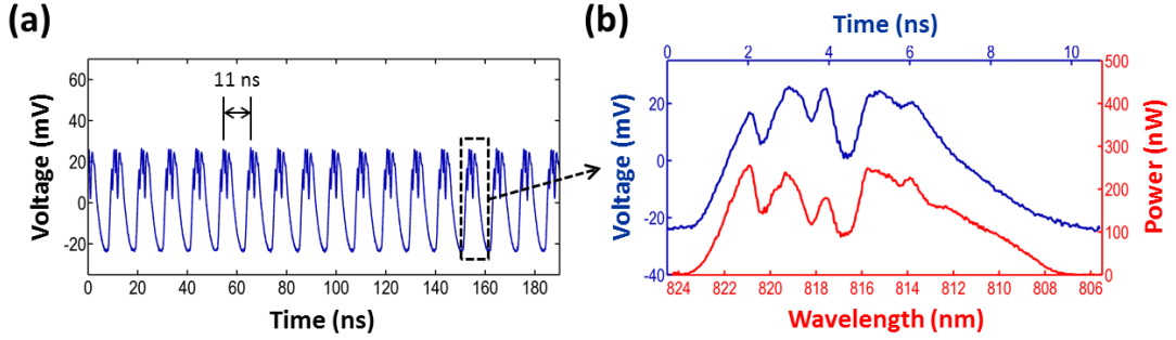
Figure 3.3: Wavelength-to-time mapping with dispersive Fourier transformation. (a) Optical pulses reflected off the target corresponding to horizontal line scans at different deflection angles of the AOD are measured by a high-speed photodetector. The period of the horizontal scans is about 11 ns, which corresponds to the mode-locked laser's pulse repetition rate (90.8 MHz). (b) Good agreement between the amplitude of the photodetector signal measured with the digitizer (shown in blue) and the power spectrum measured with a conventional optical spectrum analyzer indicates the demonstration of the wavelength-to-time mapping using the prism pairs and dispersive fiber in the 800 nm band.
