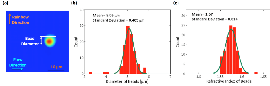
Figure 4.3: Calibration with NIST traceable beads. Polystyrene beads with a NIST traceable diameter of 5\ \mu\text{m} are used to calibrate the image processing algorithm for size measurements. (a) A custom designed image processing algorithm in CellProfiler software is used to find the beads in spatial map of optical path difference and measure the diameter. (b) Histogram of bead diameters demonstrates the measured size distribution has an expected mean of 5\ \mu\text{m} and a standard deviation within the range of optical resolution limit. (c) Since all the beads are made out of the same material, the coefficient of variation for refractive indices ( 0.014/1.57 = 0.89\% ) is much smaller than that of diameters ( 0.405/5.06 = 8.00\% ).
