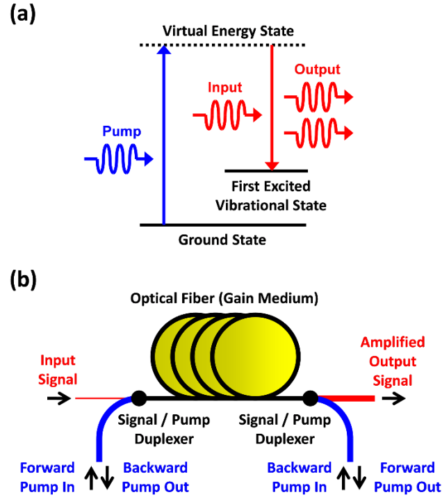
Figure 5.2: Energy diagram of stimulated Raman scattering (SRS) and basic schematic of a SRS-based optical postamplifier. (a) Raman amplification is an optical process based on the phenomenon of SRS in which the input field (called the Stokes field) stimulates the inelastic scattering of a blue-shifted pump field inside an optical medium mediated by its vibrational modes (optical phonons). (b) A typical Raman amplifier consists of a single-mode silica fiber (gain medium), an input at the Stokes frequency, and one or two pump fields that couple into and out of the fiber via duplexers such as wavelength-division multiplexers or dichroic beamsplitters. The fiber is bidirectionally pumped in the forward and backward directions to optimize the performance of the amplifier.
