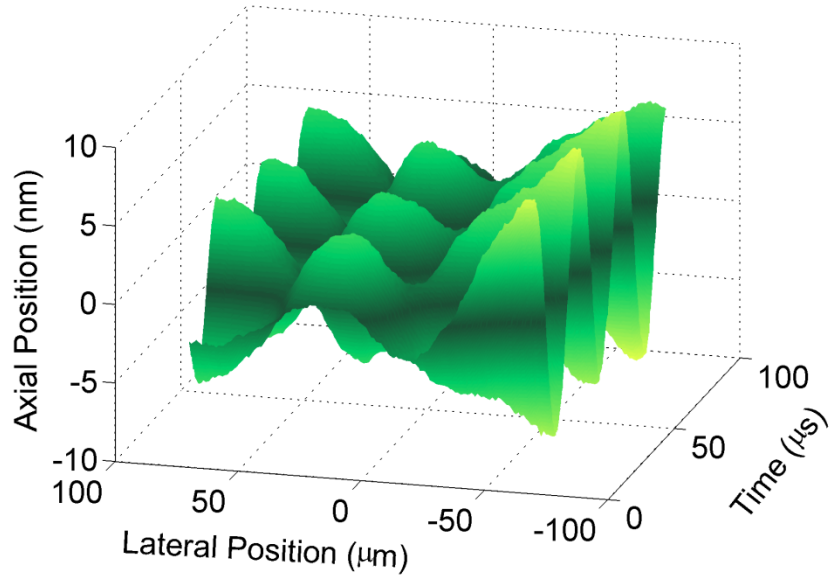
Figure 2.3: Surface vibration of the acoustic diaphragm captured by the STEAM vibrometer with \sim 1 nm axial resolution and \sim 30 ps dwell time. The diaphragm was driven to vibrate at 30 kHz.
