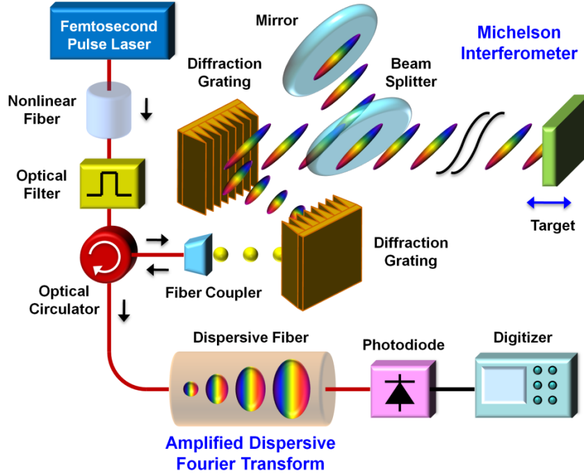
Figure 2.1: Schematic of the STEAM vibrometer. The principle of the method is three-fold: (1) encoding of the lateral and axial coordinates of the target into the different frequencies and corresponding amplitudes of a spatially dispersed broadband pulse which spectrally interferes with a reference pulse, (2) amplified dispersive Fourier transformation in which the spectrum is mapped into a temporal waveform, time-stretched so that it can be digitized in real time, and simultaneously amplified in the optical domain, and (3) Hilbert transformation on the detected pulse in the digital domain to extract the axial information of the target.
