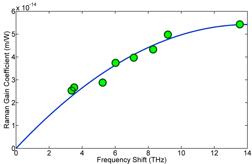
Figure 6.3: Raman gain spectrum at 808 nm Stokes wavelength. At a pump wavelength about 30 nm from the Stokes wavelength (or a frequency shift of 14 THz), the Raman gain reaches a maximum of 5.4 \times 10^{-14} m/W.
