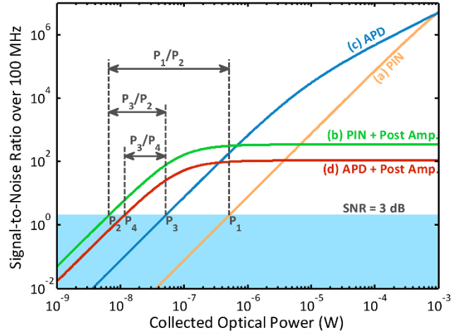
Figure 5.4: SNR over 100 MHz bandwidth for various detection methods. (a) a positive–intrinsic–negative (PIN) photodiode without a postamplifier, (b) a PIN photodiode with a postamplifier, (c) an avalanche photodiode (APD) without a postamplifier, and (d) an APD with a postamplifier. Comparing (a) and (b), the use of the postamplifier improves the sensitivity of the photodiode detection system by P_1/P_2 = 19.4 \text{ dB} . Comparing (b) and (c), the combination of the postamplifier and the photodiode is better in sensitivity than an APD alone by P_3/P_2 = 9.1 \text{ dB} .
