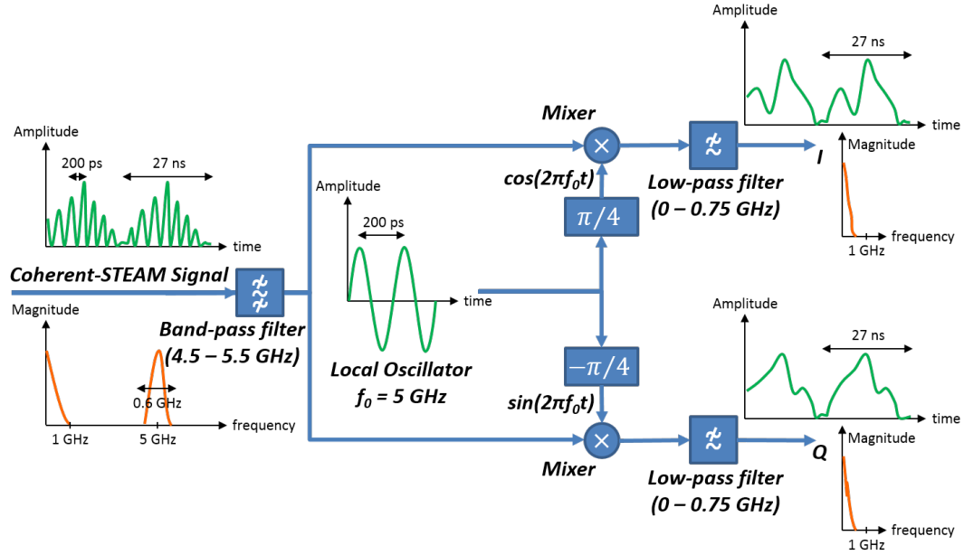
Figure 7.2: Analog preprocessing of Coherent-STEAM signal. The analog signal processing system for reducing the data rate of Coherent-STEAM is essentially a quadrature down-conversion unit. I and Q outputs and their corresponding spectra show that the down-conversion is effective in reducing the bandwidth and the required sampling rate.
