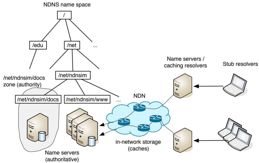
Figure 3.1: NDNS system overview
