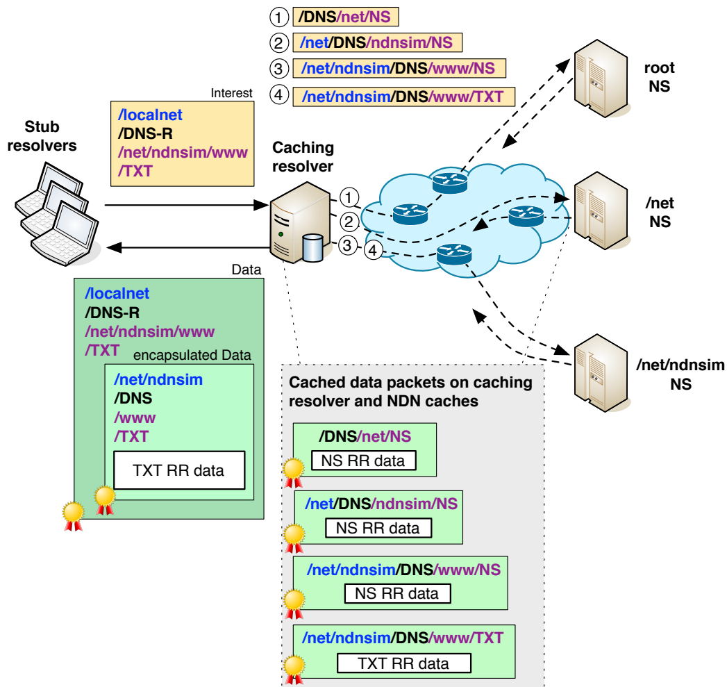
Figure 3.11: Example of DNS recursive and iterative query
