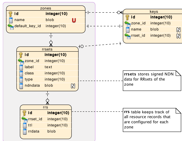
Figure 3.12: Database schema for the NDNS prototype of the authoritative name server
