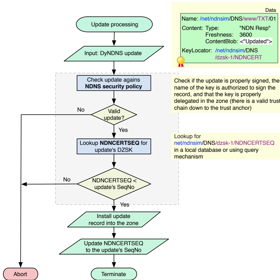
Figure 4.9: DyNDNS replay attack prevention mechanism
