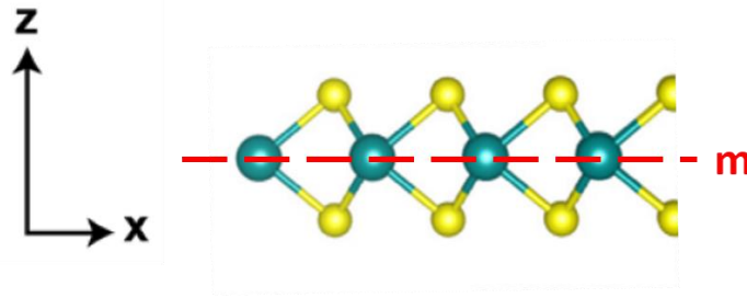
Figure 1.2: Mirror symmetry in a crystal lattice. This is a side view of crystal structure of monolayer MoS 2 . Yellow balls represent for sulfur atoms while green balls represent for Mo atoms. A mirror plane is labeled by “m” and indicated by the red dashed line. This mirror plane divides the lattice into two halves and one half is the mirror image of the other half. Therefore, this lattice has mirror symmetry (more specifically, it is out-of-plane mirror symmetry).
