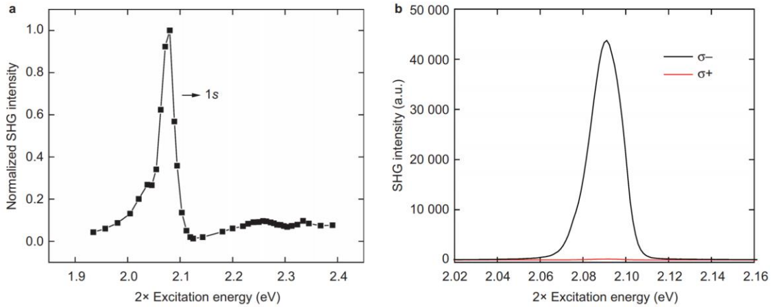
Figure 2.10: Experimental observation of the SHG selection rule in monolayer WS 2 . a , SHG intensity (black dots) versus SHG excitation energy in a scan from 0.97 eV to 1.19 eV. A dominant SHG intensity peak is observed at a pump energy of 1.045 eV, which is attributable to the 1s resonance. b , Polarization-resolved SHG measurements for \sigma_+ (red curve) and \sigma_- (black curve) detection under pumping by \sigma_+ . A negative helicity of P = -99.0\% \pm 0.1\% was observed from multiple repeated measurements. The excitation energy was 1.045 eV. The significant negative helicity at the 1s resonance confirms the existence of a rigorous selection rule for SHG. The measurement was done at 20 K
