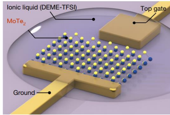
Figure 5.4: Schematics and measurement configuration. A monolayer of \text{MoTe}_2 is exfoliated onto a silicon wafer covered with a silicon oxide layer. The \text{MoTe}_2 monolayer is anchored by a ground indium/gold electrode; an isolated indium/gold pad nearby is the top-gate electrode, controlling the gate bias. A drop of ionic liquid (N,N-diethyl-N-(2-methoxyethyl)-N-methylammonium bis(trifluoromethylsulphonyl-imide), DEME-TFSI) covers the monolayer and the electrodes. This ionic liquid can manipulate the electron population in \text{MoTe}_2 , resulting in a structural transition between the 2H and 1T' phases. All devices were measured in vacuum and at 220 K.
