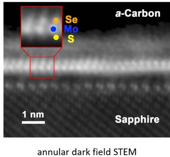
Figure 4.6: Annular dark-field scanning TEM image of the sample cross-section. It shows the asymmetric MoSSe monolayer structure with Se (orange) on top and S (yellow) at the bottom of the Mo atoms (blue).
