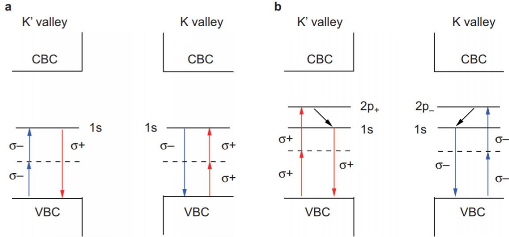
Figure 2.7: Schematics of optical selection rules based on valley-exciton locking. a , 1s exciton-resonant SHG in K' (or +K) and K (or -K) valleys. Pumped by a \sigma_+ (or \sigma_- ) polarized fundamental photon, an electron in the valence band at a K (or K') valley reaches a virtual state. Within the lifetime of the virtual state, a second \sigma_+ (or \sigma_- ) photon pumps the electron from the virtual state to the real 1s state in the K (or K') valley. Immediately, a second-harmonic photon with a \sigma_- (or \sigma_+ ) polarization is emitted. b , 2p exciton-resonant TPL in K' and K valleys. Under two-photon excitation by \sigma_+ (or \sigma_- ) polarized photons, the system transitions from the ground state to the real 2p_+ (or 2p_- ) state with a change of +1\hbar (or -1\hbar ) in the EAM at a K' (or K) valley through an intermediate virtual state. The 2p exciton relaxes to the 1s excitonic state and emits a \sigma_+ (or \sigma_- ) photon. The conduction band continuum and valence band continuum are labeled as CBC and VBC, respectively. The solid lines represent real
