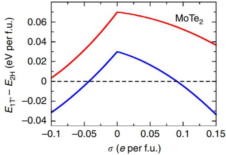
Figure 5.3: Phase boundary at constant charge in monolayer MoTe 2 . Semiconducting 2H-MoTe 2 is a stable phase and semimetallic 1T'-MoTe 2 is metastable when the monolayer is charge neutral. However, 1T'-MoTe 2 is more thermodynamically favorable when the monolayer is charged beyond the positive or negative threshold values. Reprinted with permission from [162]. Copyright Nature Publishing Group.
