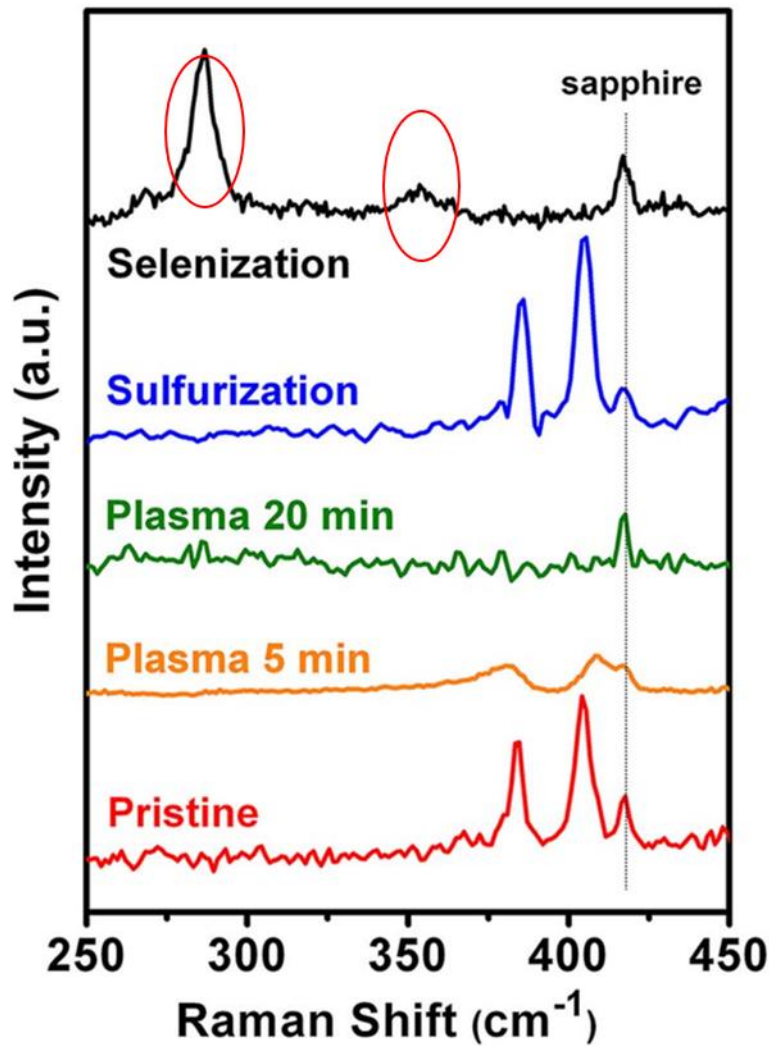
Figure 4.3: Raman characteristics at each synthesis step. It includes the \text{MoS}_2 and those after \text{H}_2 plasma treatment, sulfurization and selenization.
