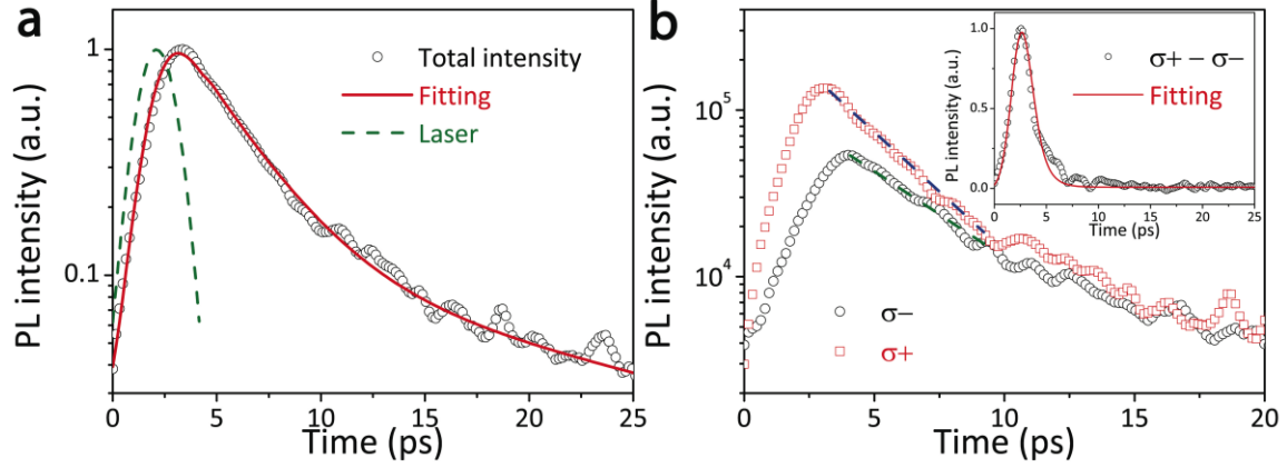
Figure 3.8: Valley dynamics measurement in monolayer WS 2 on (Ga,Mn)As. a , Time-resolved total photoluminescence using a \sigma_+ polarization femtosecond excitation laser pulse with an energy of 2.21 eV. Convolution fitting with the laser pulse (green dashed line), yields two exciton lifetimes of 2.9 ps and 20.0 ps. b , Time-resolved \sigma_+ and \sigma_- photoluminescence components excited by a \sigma_+ polarized laser. Blue and green lines indicate the different decay rates for these two components. Inset: Convolution fitting (red curve) for the time-resolved valley exciton population ( \sigma_+ - \sigma_- , black circles). The intervalley scattering time is estimated to be 2.5 ps.
