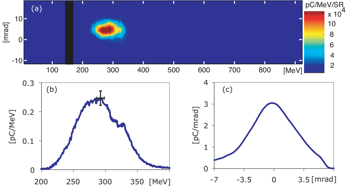
Figure 4.6: A single-shot e-beam spectrum from the 190\ \mu\text{m} diameter capillary-guided accelerator with a density of \simeq 3.2 \times 10^{18}\ \text{cm}^{-3} . (a) Image of the electron beam in pC/MeV/steradian (SR), with the energy on the horizontal axis and the divergence on the vertical axis. (b) The space-integrated spectrum of the beam in pC/MeV. (c) Energy-integrated spatial profile of the beam in pC/mrad. The peak energy was 273 MeV, total charge was \simeq 15 pC, and the beam divergence was 2.3 mrad (rms). The energy spread of the beam was estimated to be 10% (rms) with resolution of 0.77% (rms). The horizontal error bar in (b) ( \pm 5.9 MeV) comes from the uncertainty in the energy ( \pm 0.022 , see Fig. 3.7). The vertical error bar in (b) is from the uncertainty in calibration of the phosphor screen as a charge monitor ( \pm 6.8\% ). For this particular shot, the input laser energy was 1.0 J with pulse duration of 46 fs, which gave the input laser power of 22 TW ( a_0 \simeq 1.1 ). The maximum charge density on the LANEX-FB was < 0.04\ \text{pC}/\text{mm}^2 .
