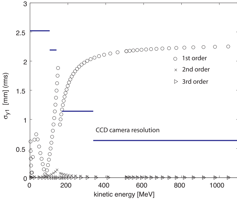
Figure 3.5: Calculated contributions to the vertical beam size of each order. Assumed input beam is a Gaussian distribution with \sigma_{x0} = \sigma_{y0} = 20 \mu\text{m} (rms), and \sigma_{x'0} = \sigma_{y'0} = 2 \text{ mrad} (rms). Horizontal axis is the kinetic energy of electron for a peak magnetic field of 1.25 T. Also shown are spatial resolutions of CCD cameras.
