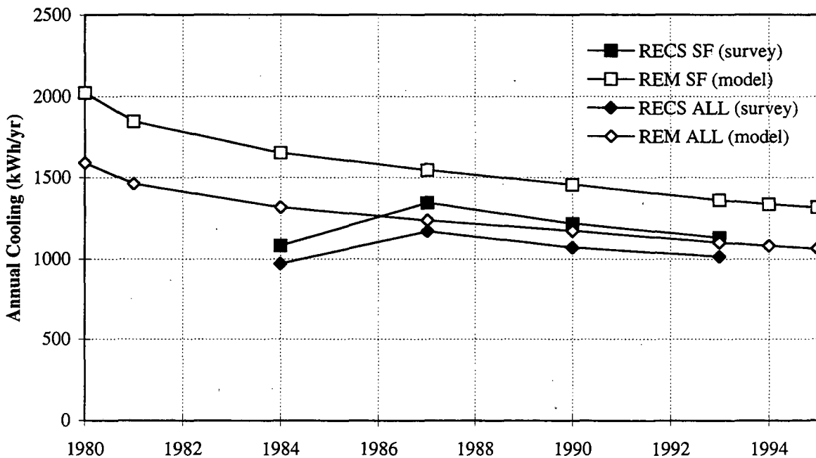
Figure 3.10. National Average Room Air Conditioner (RAC) UEC (per household)
