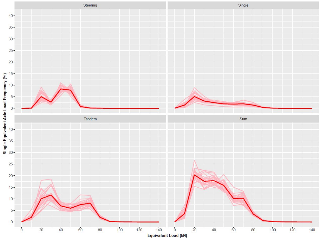
Figure 3.17: Axle loads Spectra 3.
