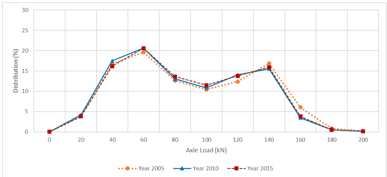
Figure 3.2: WIM axle load spectra of tandem axles for 2005, 2010, and 2015.
