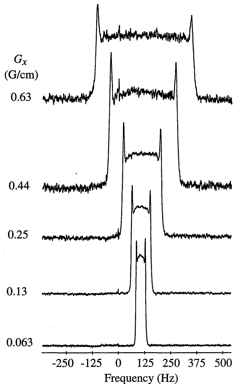
Figure 7.7: 1-D ^{129}\text{Xe} MR images taken as a function of applied gradient along \bar{x} , obtained with G_x = 0.063, 0.13, 0.25, 0.44, 0.63 G/cm [201]. These images depict the evolution of the lineshape with increasing gradient strength in the weak-diffusion regime. Note the pronounced edge-enhancement effects.
