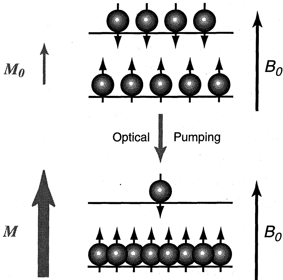
Figure 2.1: Cartoon depicting the effect of laser-polarization for a collection of spin- 1/2 nuclei (assuming positive gyromagnetic ratio). Normally, the number of spins aligned antiparallel to the magnetic field ( B_0 ) is nearly equal to the number of spins aligned with B_0 , leading to a tiny detectable magnetization, M_0 . However, with optical pumping, the population distribution of the spins can be driven far away from equilibrium, thereby increasing the magnetization to order unity. Figure adapted from Ref. [17].
