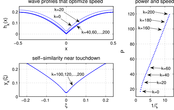
FIGURE 6. Upper left: the optimal curves h_k(x) approach the periodic parabola \sqrt{6}\ell_0(|x| - x^2) as \delta_k \rightarrow 0 . Lower left: the curves appear to be self-similar when scaled using (4.6); the curves shown lie in the range 1.4 \times 10^{-4} \geq \delta_k \geq 1.0 \times 10^{-7} . Right: as \delta_k \rightarrow 0 , the swimming speed V \approx \frac{3}{2} - \frac{3}{8}\zeta approaches \frac{3}{2} while the power required to swim at that speed grows without bound.
