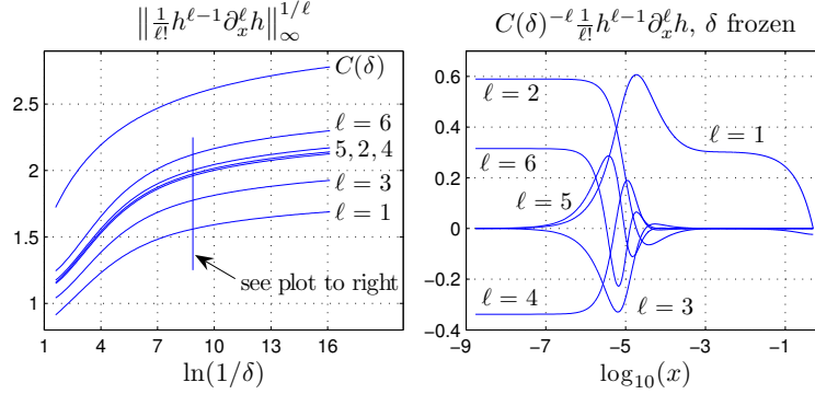
FIGURE 18. Left: plot of the quantities in (C 20) vs. \ln(1/\delta) together with the common bound C(\delta) defined after (C 20) for the optimal solutions of Problem 1 in Section 3. Right: plot of the functions C(\delta)^{-\ell} \frac{1}{\ell!} h(x)^{\ell-1} \partial_x^\ell h(x) for 1 \leq \ell \leq 6 over the range 10^{-9} \leq x \leq 0.5 with \delta = \delta_{100} = 1.41 \times 10^{-4} held fixed. The \ell th roots of the absolute maxima in this plot correspond to the values at the cross section shown in the left plot, divided by C(\delta) .
