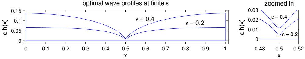
FIGURE 15. Wave profiles identified in Figure 14 as optimal when corrections through fourth order in \varepsilon are included in the calculation of speed and efficiency.
