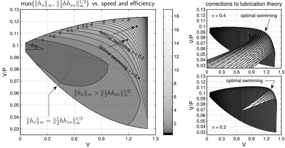
FIGURE 14. Left: Maximum slope and square root of maximum “gap-weighted curvature” of solutions of Problem 3, re-scaled for constant fluid loss ( Z[h] = 0.2 ). These quantities dictate how small \varepsilon = H/W must be for the lubrication approximation to remain valid. For smaller values of \varepsilon , (V, V/P) can approach the theoretical maximum (1.5, 0.15) more closely without leaving the realm of lubrication theory. Right: If corrections through fourth order in \varepsilon are included, the attainable region “folds over” itself, penalizing wave profiles that are too cusp-like.
