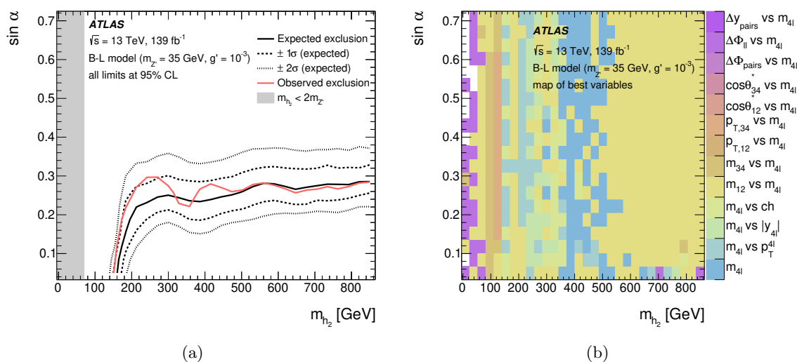
Figure 13. (a) Exclusion contour at 95% confidence level for the B - L gauge model [104] in the plane of \sin \alpha versus m_{h_2} for m_{Z'} = 35 GeV and g' = 10^{-3} . The red line shows the observed exclusion and the solid black line shows the expected exclusion, with the dashed black lines indicating the \pm 1\sigma and \pm 2\sigma uncertainty bands. The region above and to the left of the lines is excluded, up to the grey band, which shows the region m_{h_2} < 2m_{Z'} , where the four-lepton final state has no sensitivity. (b) Colour palette indicating which observable has the highest expected sensitivity at each point in the parameter space and is used to set the limit.
