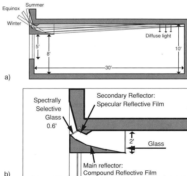
Figure 2. South-facing light shelf: (a) Section along centerline of room, and (b) detail of light shelf reflectors.
