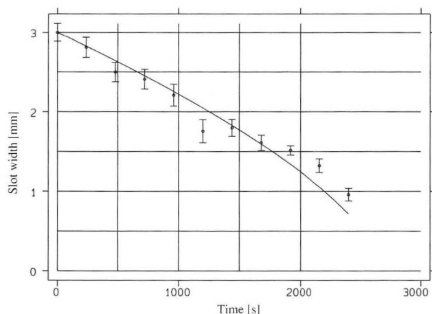
Figure 1. Predicted (solid line) and measured slot width over the course of the sealing process for a 3 mm by 40 mm leak.
