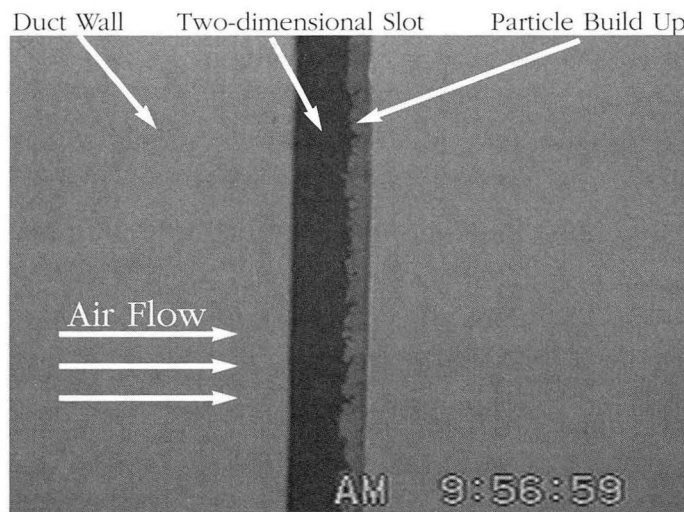
Figure 2. Top view of a 3 mm by 40 mm slot after 20 minutes of injection.
