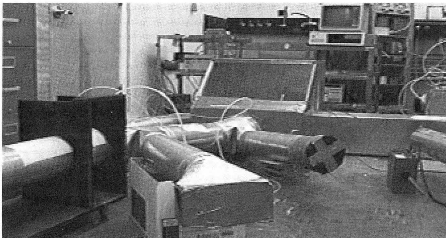
Figure 4. Video-frame capture of the apparatus used to test aerosol sealant effectiveness.
