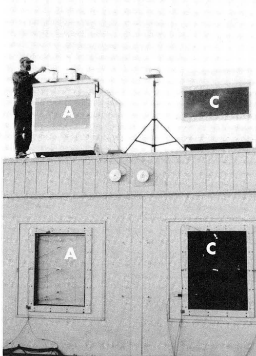
Figure 1. This "smart" automated venetian blind system has been designed to respond to changing solar conditions and access to view in real-time by using a network of sensors and an intelligent computer control system to operate the slat angle of the blinds. In this field test, we are comparing the thermal performance of the smart system (left) to a static tinted glazing system (right) using the Mobile Window Thermal Test (MoWiTT) facility.
