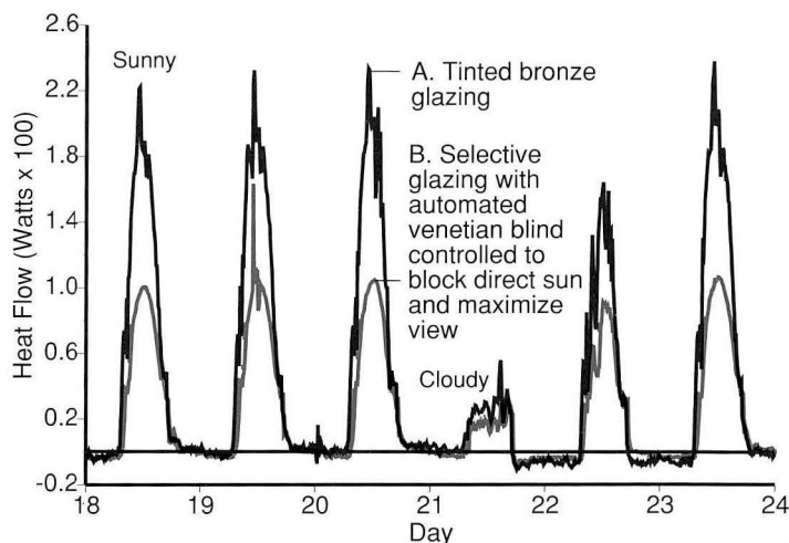
Figure 3. Results from the MoWiTT facility for a clear day indicate that the automatically controlled interior blind coupled with a selective glazing system (B) was more than twice as effective at reducing solar heat gain as a commonly used nonoperable system, single-tinted (bronze) glazing (A), while providing approximately the same electric light energy savings. The large differences in the heat flow between the two samples were driven principally by the admittance of direct sun into the base-case chamber.
