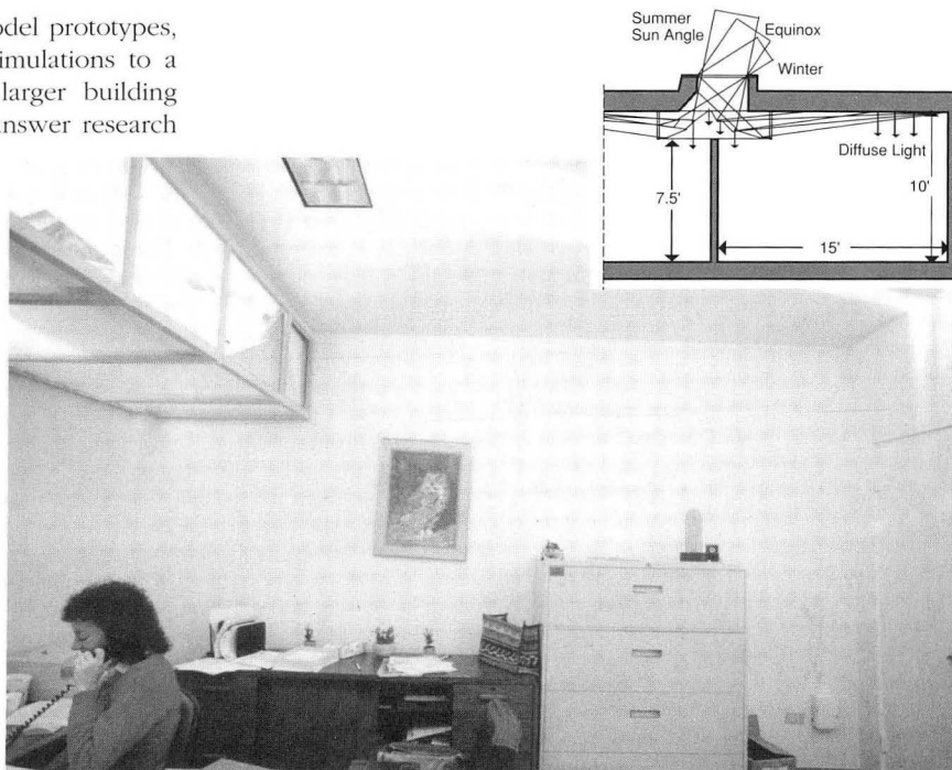
Figure 4. The reflector system used in the prototype skylight for the Palm Springs Chamber of Commerce was designed to split the incoming daylight flux and redirect it to the ceiling plane of two separate rooms (see inset diagram). The installed skylight (above) yielded excellent illuminance uniformity on the workplane and brightened typically dark wall and ceiling surfaces.
