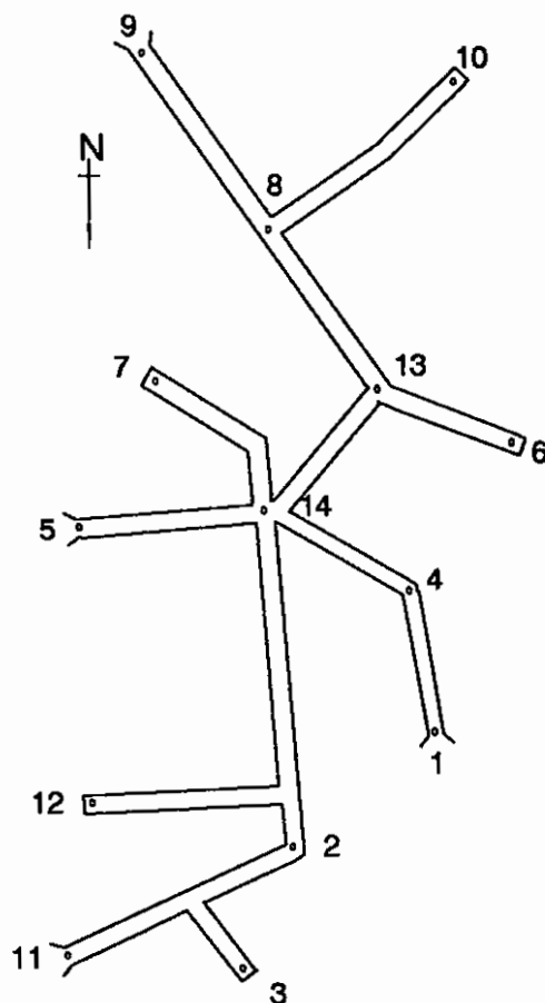
Figure 1. Plan of artificial warren showing location of 14 gas sampling points.
