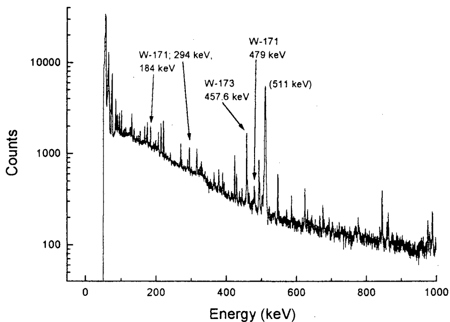
Figure 4-9(b): \gamma -Spectrum of second count for the collection shown above in (a).
