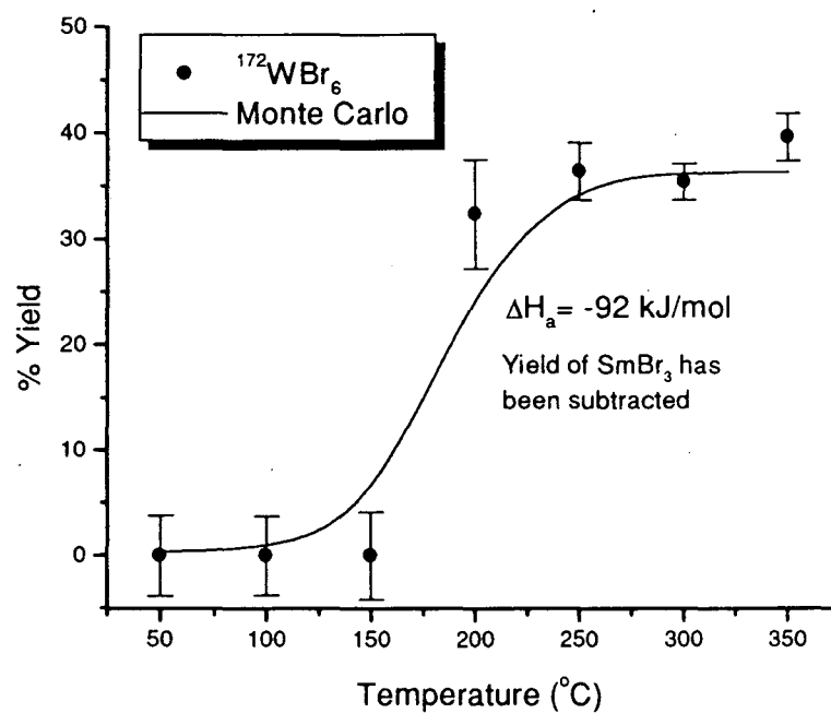
Figure 5-19: Corrected volatility and calculated adsorption enthalpy curve for ^{172}\text{WBr}_6 .
