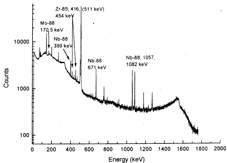
Figure 4-10(a): \gamma -Spectrum of Yield Check collection for the ^{nat}\text{Cu}(^{28}\text{Si}^{6+}, \text{pxn})^{88,89}\text{Mo}, ^{88}\text{Nb}, ^{85}\text{Zr} reaction.
