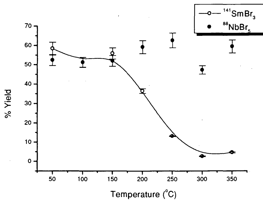
Figure 5-13(a): Observed yield as a function of temperature for ^{88}\text{NbBr}_5 and ^{141}\text{SmBr}_3 .
