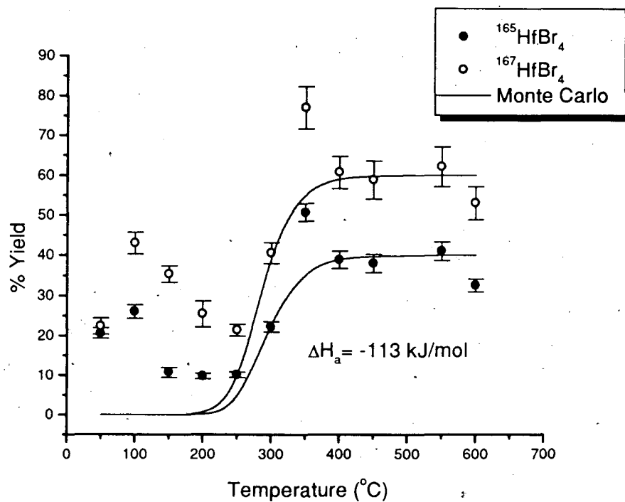
Figure 5-6: Volatility and calculated adsorption enthalpy curves for ^{165,167}\text{HfBr}_4 from the reaction ^{\text{nat}}\text{Eu}(^{19}\text{F}^{5+}, x\text{n})^{165-167}\text{Hf} .
