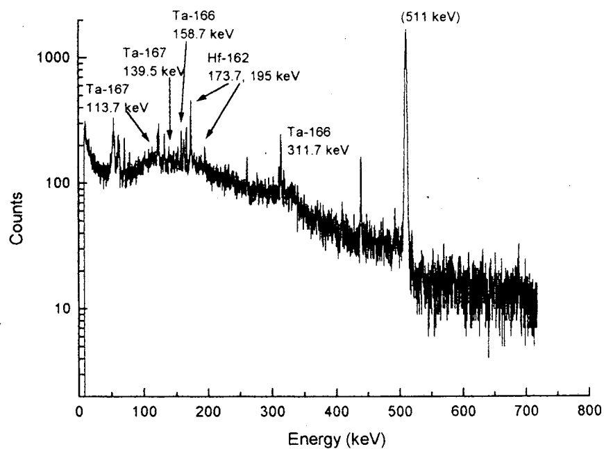
Figure 4-7 (b): \gamma -Spectrum of Gas Chromatography collection for the ^{147}\text{Sm}/^{nat}\text{Eu}(^{20}\text{Ne}^{6+}, xn)^{162}\text{Hf}, ^{166,167}\text{Ta} reaction. Temp. = 500° C.
