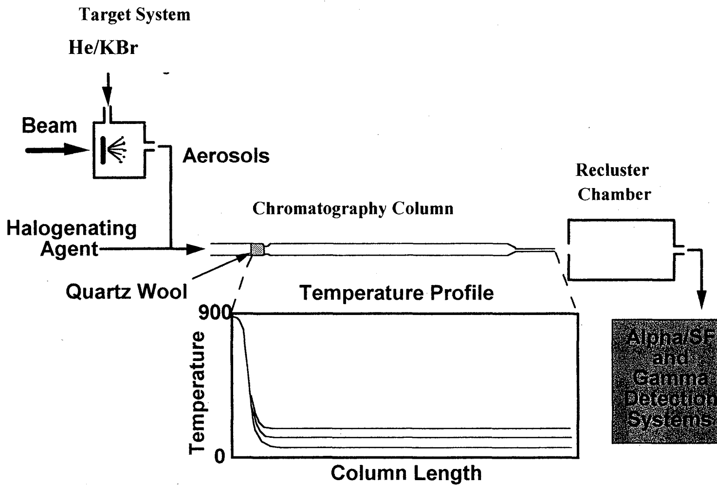
Figure 3-1: Schematic of the Heavy Element Volatility Instrument (HEVI).
