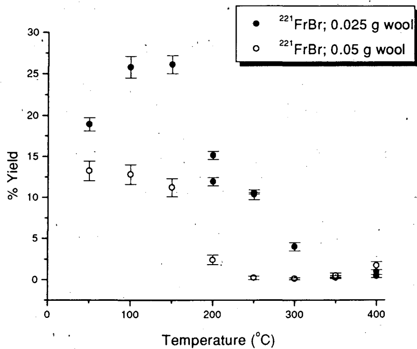
Figure 5-2: Yield of the 4.8-min ^{221}\text{FrBr} between 0^{\circ} and 400^{\circ}\text{C} , with 150 ml/min HBr flow and a variable mass of quartz wool.
