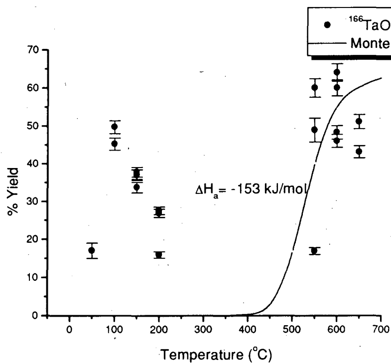
Figure 5-14: Volatility and calculated adsorption enthalpy curves for ^{166}\text{TaOBr}_3 . From the reaction ^{\text{nat}}\text{Eu}(^{20}\text{Ne}^{6+}, \text{xn})^{166-167}\text{Ta} .
