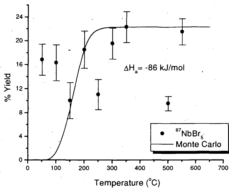
Figure 5-12: Volatility and calculated adsorption enthalpy curves for ^{87m}\text{NbBr}_5 . From the reaction ^{\text{nat}}\text{Cu}(^{28}\text{Si}, \alpha xn)^{87m}\text{Nb} .
