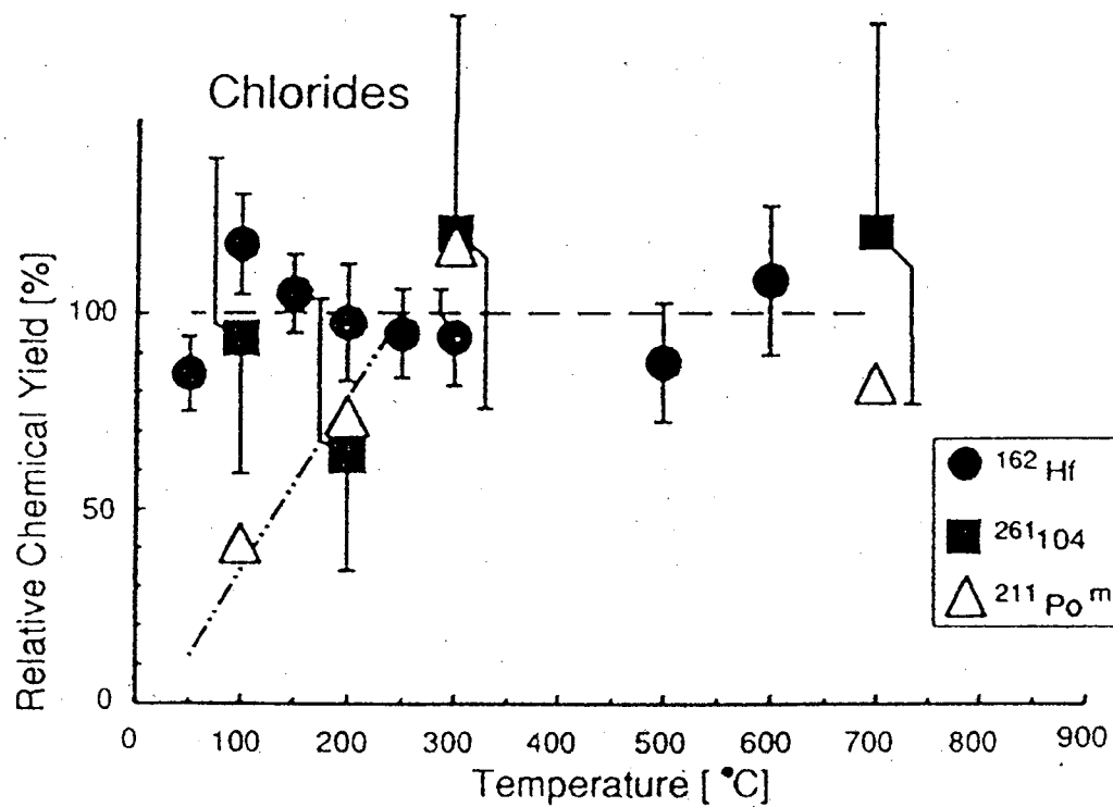
Figure 5-22: Results of OLGA II experiments with Chlorides of Po, Hf, and Rf.
