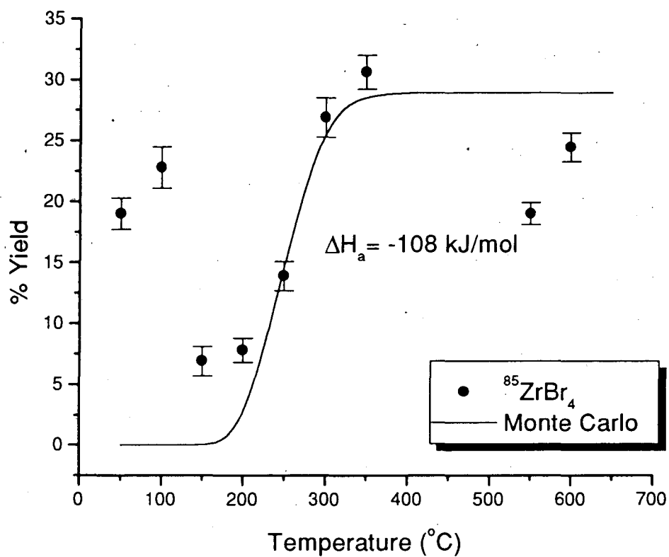
Figure 5-5: Volatility and calculated adsorption enthalpy curve from the Monte Carlo program for ^{85}\text{ZrBr}_4 , from the reaction ^{\text{nat}}\text{Cu}(^{28}\text{Si}, 3\text{p}3\text{n})^{85}\text{Zr} . Data are taken from the second count of each collection.
