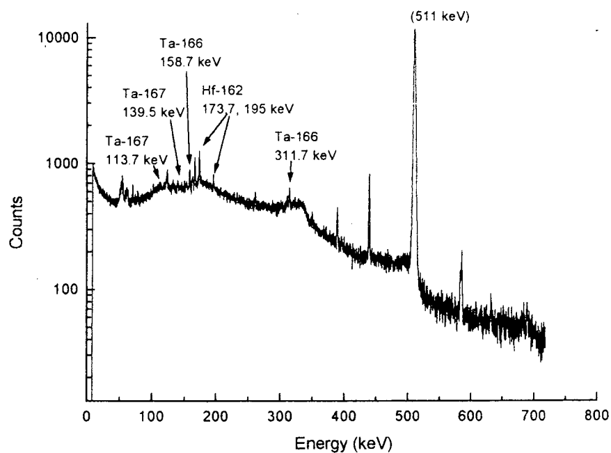
Figure 4-7 (a): \gamma -Spectrum of Yield Check collection for the ^{147}\text{Sm}/^{nat}\text{Eu}(^{20}\text{Ne}^{6+}, xn)^{162}\text{Hf}, ^{166,167}\text{Ta} reaction.
