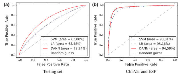
Fig. 1. ROC curves comparing performances of the neural network (DANN), support vector machine (SVM), and logistic regression (LR) models in discriminating (a) 'simulated' variants from 'observed' variants in the testing set and (b) pathogenic ClinVar variants from likely benign ESP alleles (DAF \geq 5\% )
