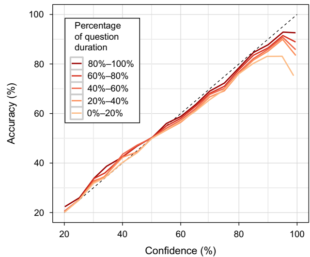
Figure 1. (Color online) Calibration Curves, Conditional on When in the Question's Life the Forecast Was Made
