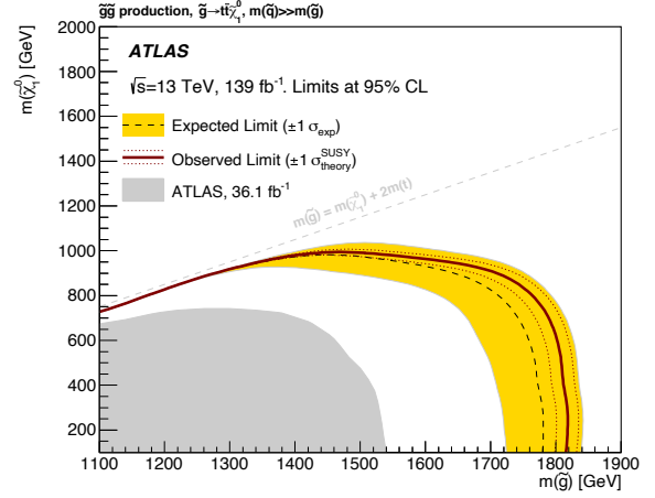
(b) \tilde{g} \rightarrow t\tilde{\chi}^0_1
