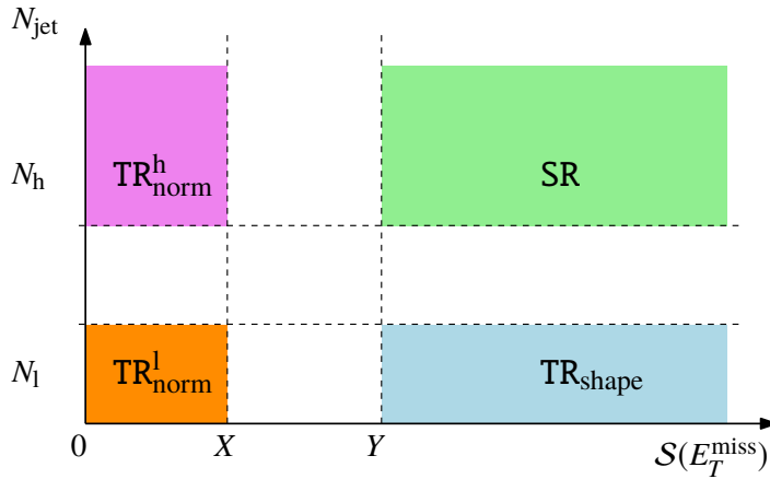
Figure 2: Schematic of the kinematic regions used in the multijet template estimate for the multijet background. SR represents any signal region, while the three TR variations are regions used to extract and normalise the corresponding background prediction.
