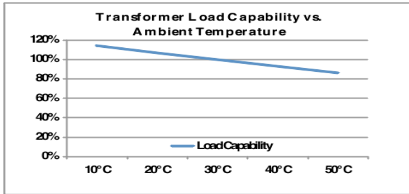
Figure 7. Change in Transformer Capacity as a Function of Ambient Temperature
