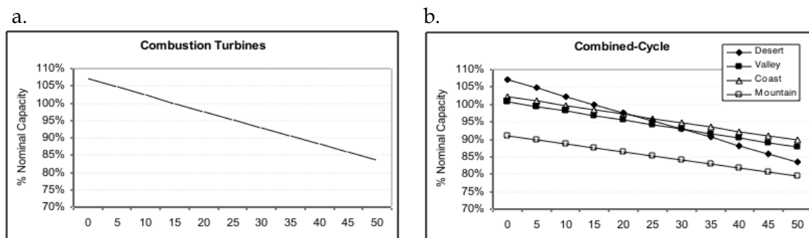
Figure 3. Change in Turbine Capacity as a Function of Ambient Temperature
