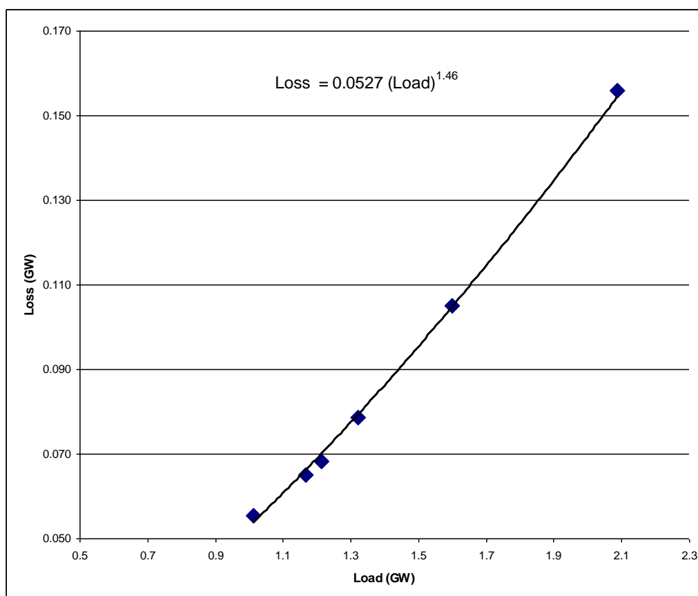
Figure 10. System Load and System Losses
