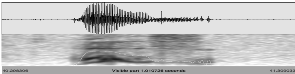
Figure 5: Waveform and spectrogram for /ad/
