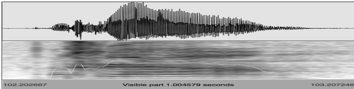
Figure 14: Waveform and spectrogram for /rra/
