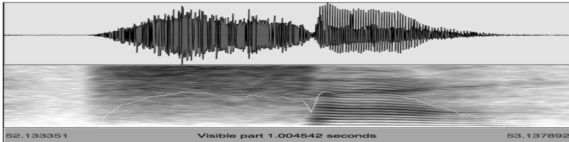
Figure 8: Waveform and spectrogram for /ffa/
