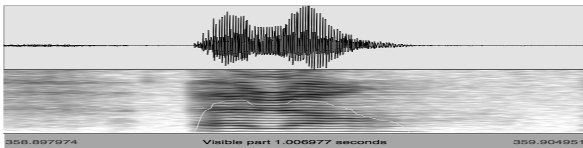
Figure 15: Waveform and spectrogram for /ala/
