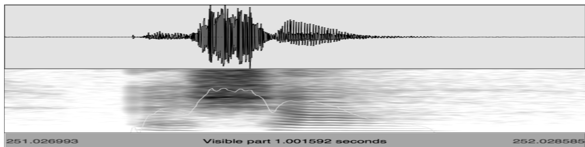
Figure 9: Waveform and spectrogram for /aʃa/
