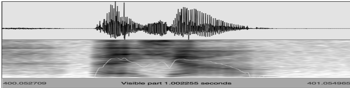
Figure 4: Waveform and spectrogram for /agga/
