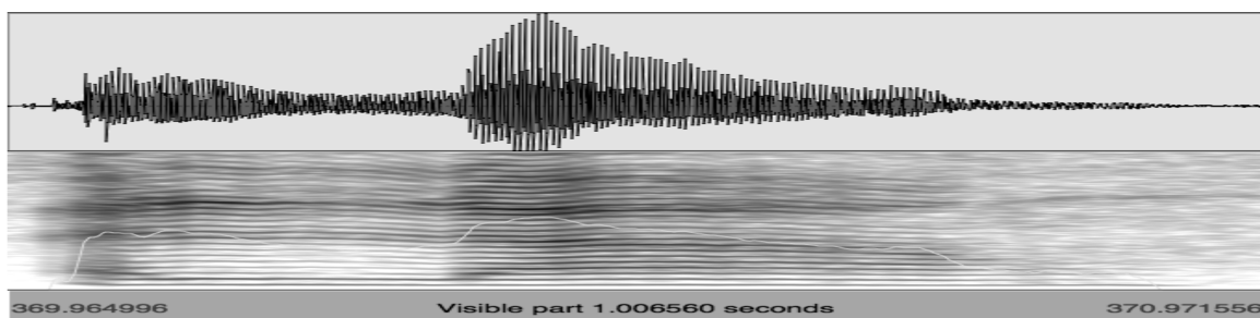
Figure 16: Waveform and spectrogram for /alla/
