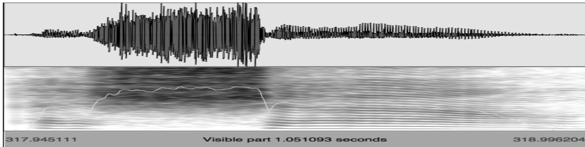
Figure 10: Waveform and spectrogram for /affa/
