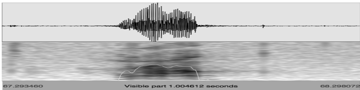
Figure 13: Waveform and spectrogram for /ra/
