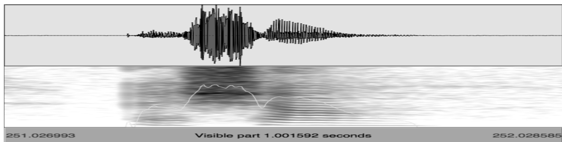
Figure 9: Waveform and spectrogram for /aʃa/
