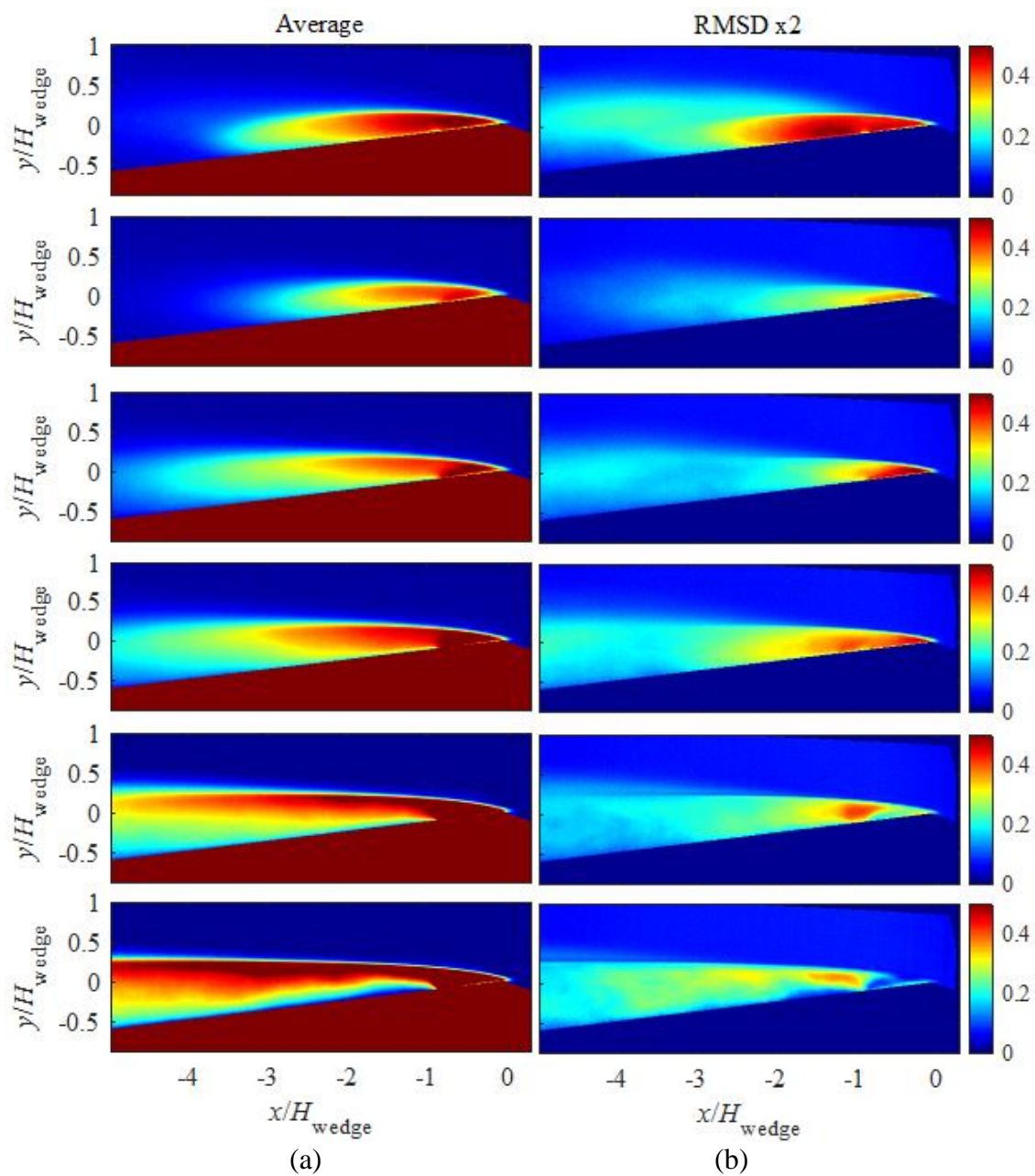
Figure 14: (a) The time-average and (b) RMSD x2 (multiplied to enable sharing color scale) of the void fraction fields for increasing rates of gas injection into the mid-cavity Q_I/Q_{V,max} = 0, 0.16, 0.32, 0.48, 0.80 and 1.20 increasing from top to bottom; \sigma_0 = 2.0 and U_0 = 8 \text{ ms}^{-1} .
