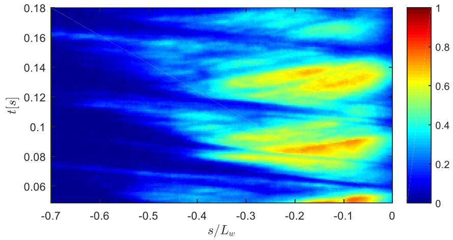
Figure 22: The s - t diagram (at n = 2 mm) for the cavity injection case (same as that shown in figures 16a-c) with Q_I/Q_{V,max} = 0.07 , \sigma_0 = 2.0 and U_0 = 8 ms ^{-1} .
