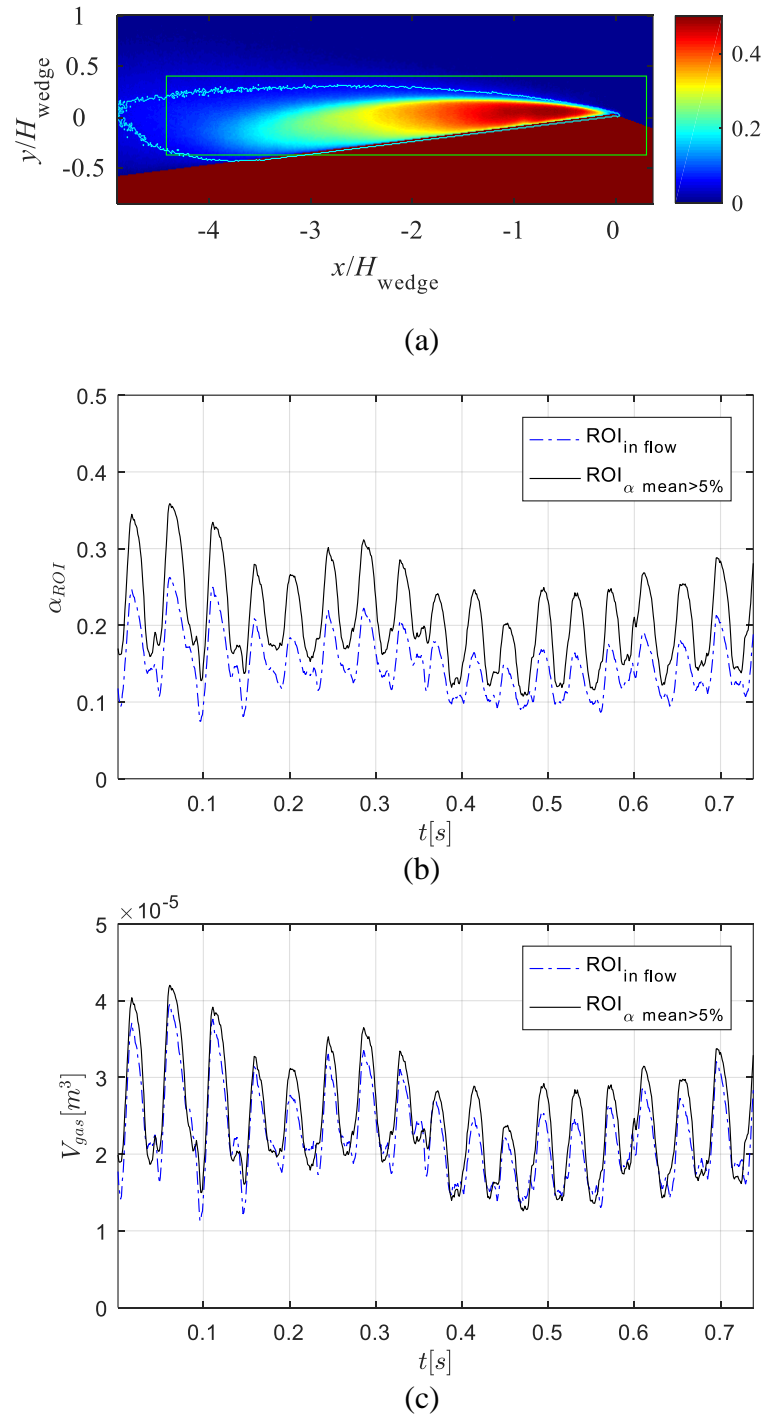
Figure 5: (a) The time-averaged void fraction distribution with outlines shown for two regions of interest (ROI); (the first ROI is rectangular and the second is based on the time-averaged 5% void fraction contour). Time-series of spatially averaged void fraction (b) and gas volume (c) within the two ROIs (outlined in (a)) for the baseline shedding cavity at \sigma_0 = 2.0 and U_0 = 8 \text{ ms}^{-1} .
