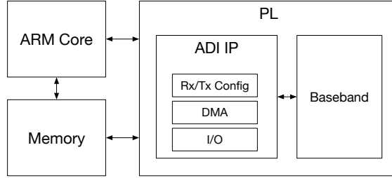
Figure 5.7. Block diagram showing custom baseband integrated on PL fabric with ADI IP.
