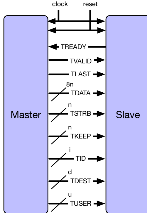
Figure 6.1. Illustration of signals in the AXI-4 Stream standard.
