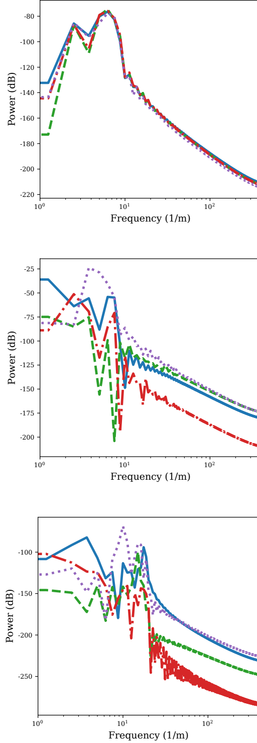
Figure 5.11. The figures above show measured power spectral densities from the VNA-based setup. Each line corresponds to a different measurement. The top figure has f_c = 915 MHz, the center has f_c = 2.45 GHz, and the bottom has f_c = 5.8 GHz. These figures originally appeared in [83].
