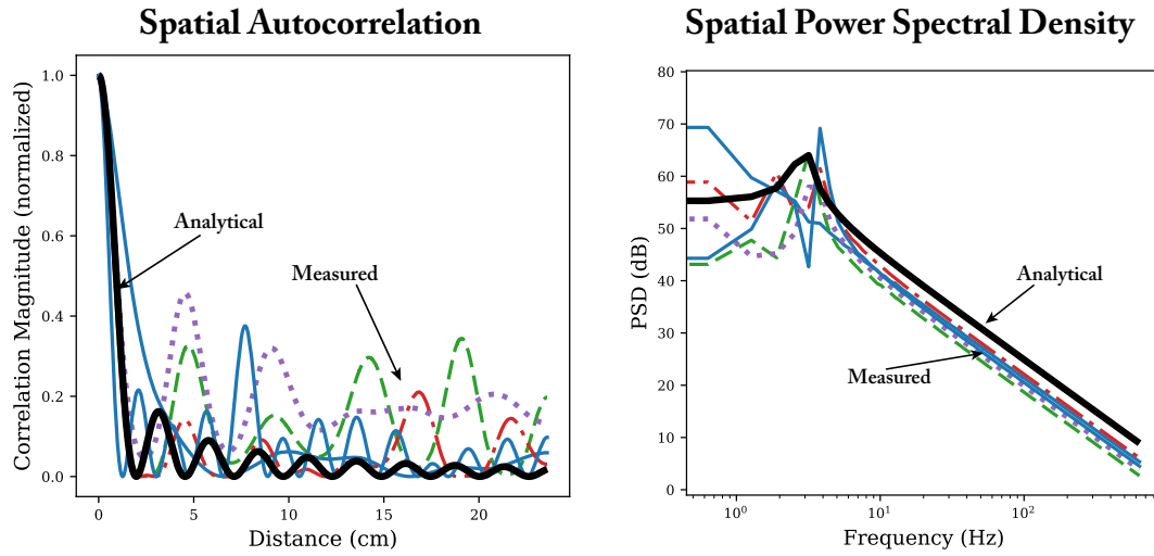
Figure 5.10. Normalized correlation and power spectral density of channel measurements at 5.8 GHz. Note that the spatial autocorrelation plot is in distance units whereas the power spectral density plot is in temporal frequency units. The scaling of the PSD plot emphasizes that the peak is at the expected frequency corresponding to the maximum Doppler shift. Both figures are normalized so that lag 0 of the correlation is 1. Bold black lines are the expected analytical result. All other lines are different measured results with the transmit antenna moved in-between measurements. These figures originally appeared in [83].
