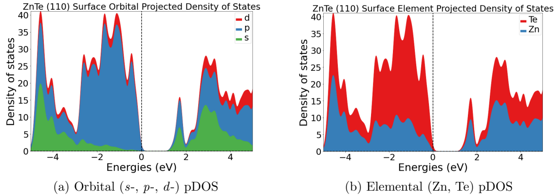
Figure 4: Projected Density of States (pDOS) at the band edges for the ZnTe (110) surface, Gaussian-smoothed ( \sigma = 0.1 ). Calculations show predominantly p -character at the VBM, and predominantly s - & p -character at the CBM. There is a high Te contribution to the VBM, whereas both Te and Zn states contribute to the CBM. This is in similar to other metal-chalcogenide semiconductors.
