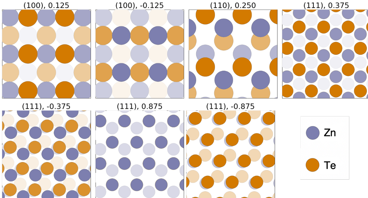
Figure 3: ZnTe surfaces generated as part of the workflow with a maximum Miller index of 1. Each surface is identified by a Miller plane and the fractional shift applied in the c direction to get to the specific termination
