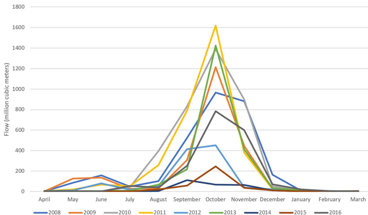
Fig. 3. E9 Gauge Flow by Month, 2008–2016.
