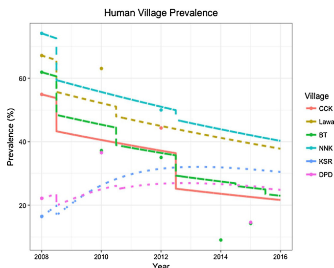
Fig. 4. Single village model with human infection survey data.
