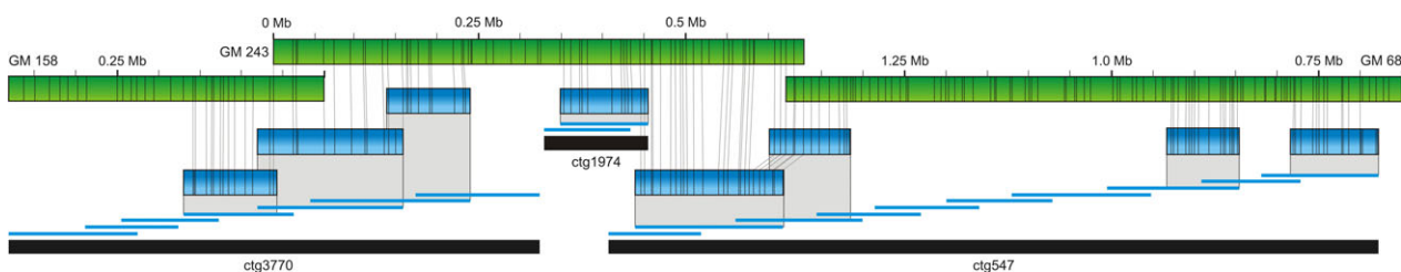
Figure 4 Merging genome maps. Three genome maps (green bars) could be merged together after aligning sequences of BAC clones (blue bars) from three contigs of the physical map (black bars).
