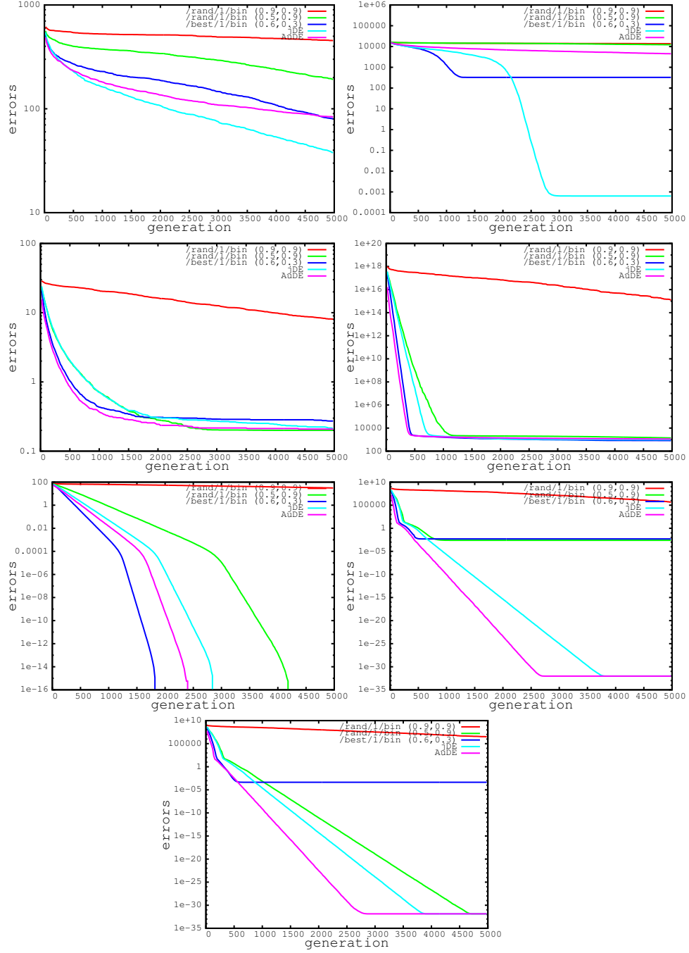
Figure 3: Evolution of the average error in the second seven test functions: top left is the Rastrigin's function, top right is the Schwefel's function, middle left is the Salomon's function, middle right is the Whitely's function, bottom left is the Weierstrass's function, bottom right is the generalized penalized function I, and last plot is the generalized penalized function II.
