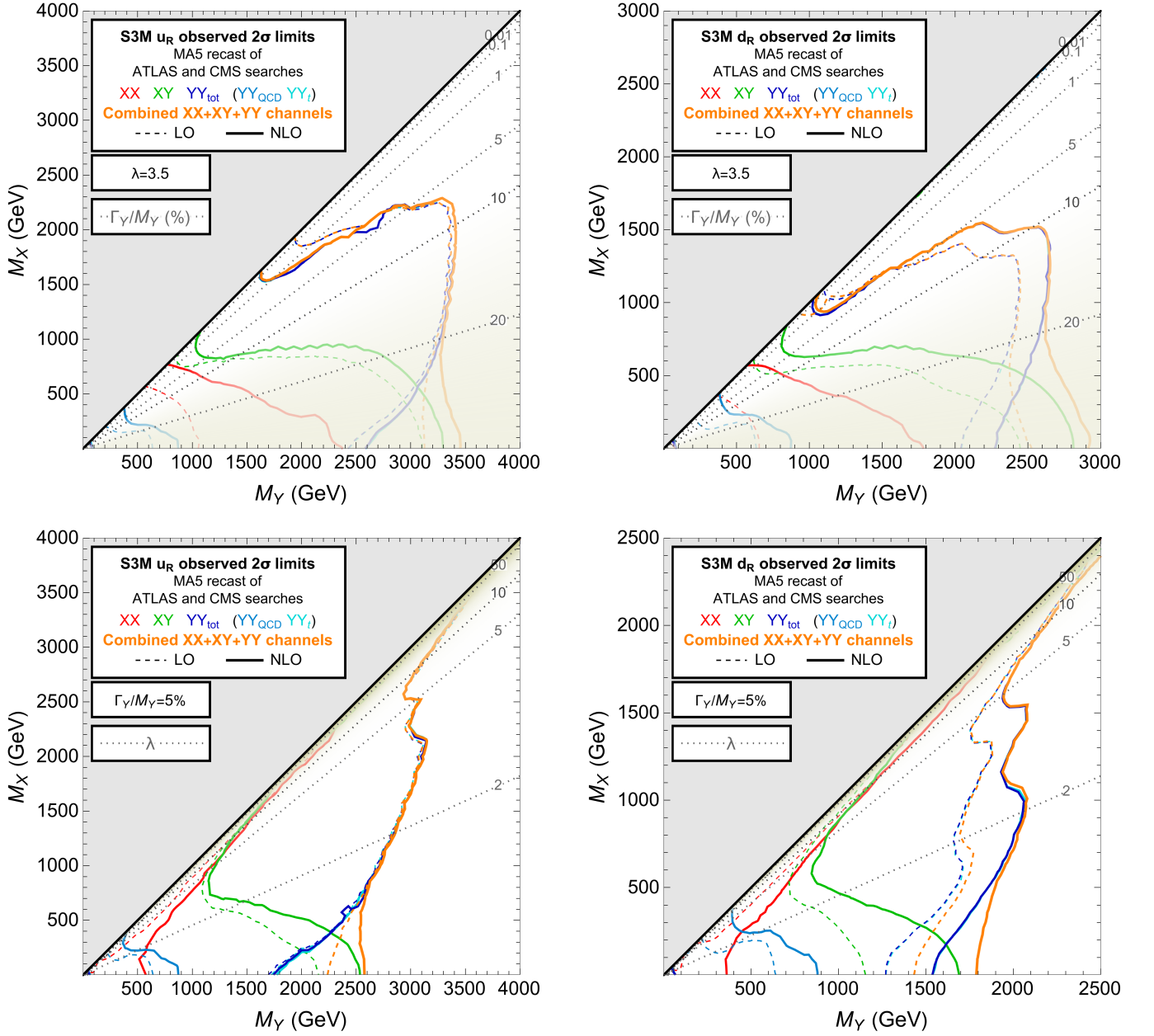
FIG. 1. Exclusion limits at 95% confidence level from the reinterpretation of several Run 2 ATLAS and CMS searches [133–137]. The results are shown for the S3M_{uR} (left) and S3M_{dR} (right) real dark matter scenarios described in section II.1, considering two configurations: \lambda = 3.5 (top row) and \Gamma_Y/M_Y = 0.05 (bottom row). For scenarios with \lambda = 3.5 , dotted grey lines represent isolines of constant \Gamma_Y/M_Y value. Conversely, for scenarios with \Gamma_Y/M_Y = 0.05 , these lines correspond to isolines of fixed \lambda value. Individual contributions to the bounds are displayed for processes XX (red), XY (green), and YY (dark blue), with the YY process further decomposed into its purely QCD part ( YY_{QCD} , teal) and its t -channel part ( YY_t , turquoise). The yellow gradient highlights regimes where either the perturbative approach becomes increasingly invalid due to large coupling values or the narrow-width approximation loses validity due to a large mediator width-to-mass ratio.
