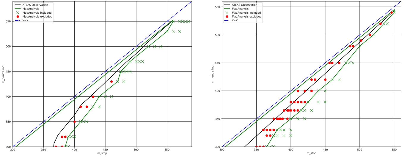
FIG. 55. Excluded region at the 95% CL, displayed in the (m_{\tilde{t}_1}, m_{\tilde{\chi}_1^0}) mass plane for the pp \rightarrow \tilde{t}_1 \tilde{t}_1^* \rightarrow (c \tilde{\chi}_1^0)(\bar{c} \tilde{\chi}_1^0) (left) and pp \rightarrow \tilde{t}_1 \tilde{t}_1^* \rightarrow (b f \tilde{f}' \tilde{\chi}_1^0)(\bar{b} f' \tilde{f}' \tilde{\chi}_1^0) (right) processes. The green crosses and red dots respectively correspond to scenarios allowed and excluded when using our implementation of the ATLAS-EXOT-2018-06 analysis in MadAnalysis 5 . The excluded parameter space regions are thus delineated by the green contours, that could be compared to the official ATLAS exclusions (black).
