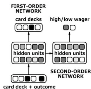
Figure 2: Network architecture for the IGT simulation.
