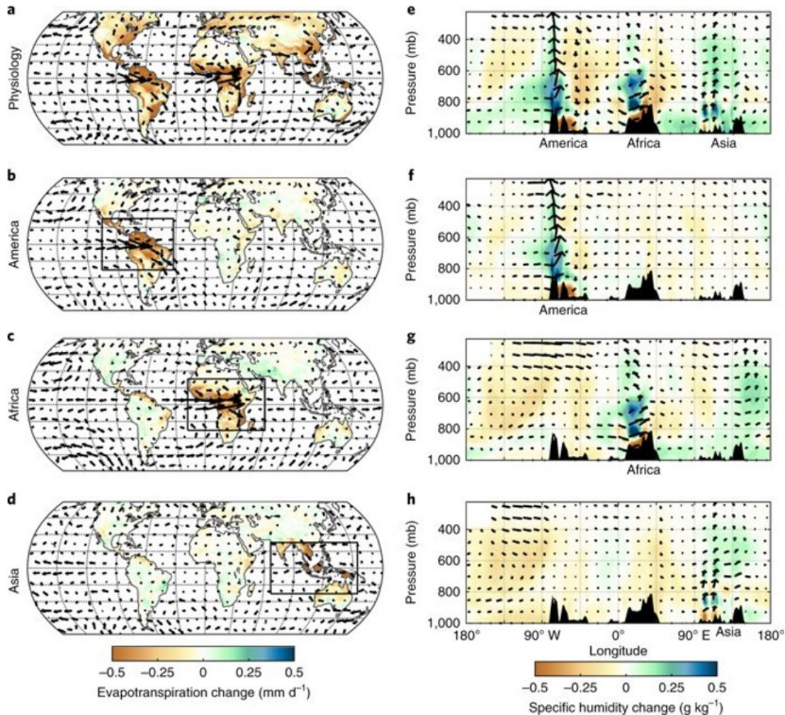
Fig. 4: Changes in evapotranspiration and specific humidity. a-h, Annual mean evapotranspiration (a-d) and tropical ( 5^\circ \text{S} - 5^\circ \text{N} ) meridional mean specific humidity (e-h) change. Changes from the CESM ( 4 \times \text{CO}_2 minus preindustrial) for the physiology (a,e), America (b,f), Africa (c,g) and Asia (d,h) simulations. Arrows in a-d show the change in 850 mb horizontal wind and arrows in e-h show the change in meridional mean zonal and vertical ( \omega ) circulation with pressure as the vertical coordinate.
