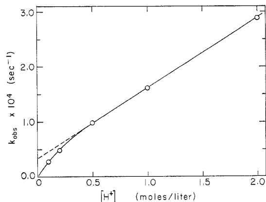
Figure 6.—Hydrogen ion dependence of the first-order rate constant for the aquation of \text{Ru}(\text{NH}_3)_6\text{py}^{2+} ; ionic strength = 2.0 \text{ M} ( \text{NaCl} ); temperature 25.0^\circ .
