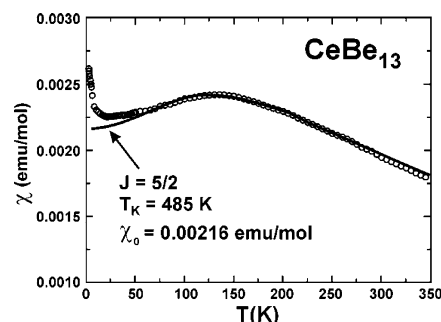
Figure 4. Magnetic susceptibility of \text{CeBe}_{13} . The large \chi and broad maximum at T_{\text{max}} \approx 130 K is typical of intermediate valence systems.
