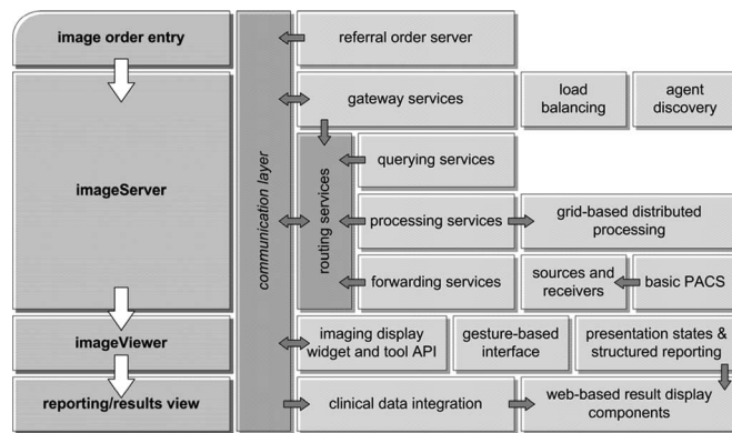
Fig. 1. Overall architecture for the openSourcePACS system, consisting of four different modules: 1) image order entry; 2) imageServer; 3) imageViewer; and 4) reporting/results viewing. A Java messaging system (JMS)-based communication layer ties together each of these parts. The submodules making up each module are depicted.
