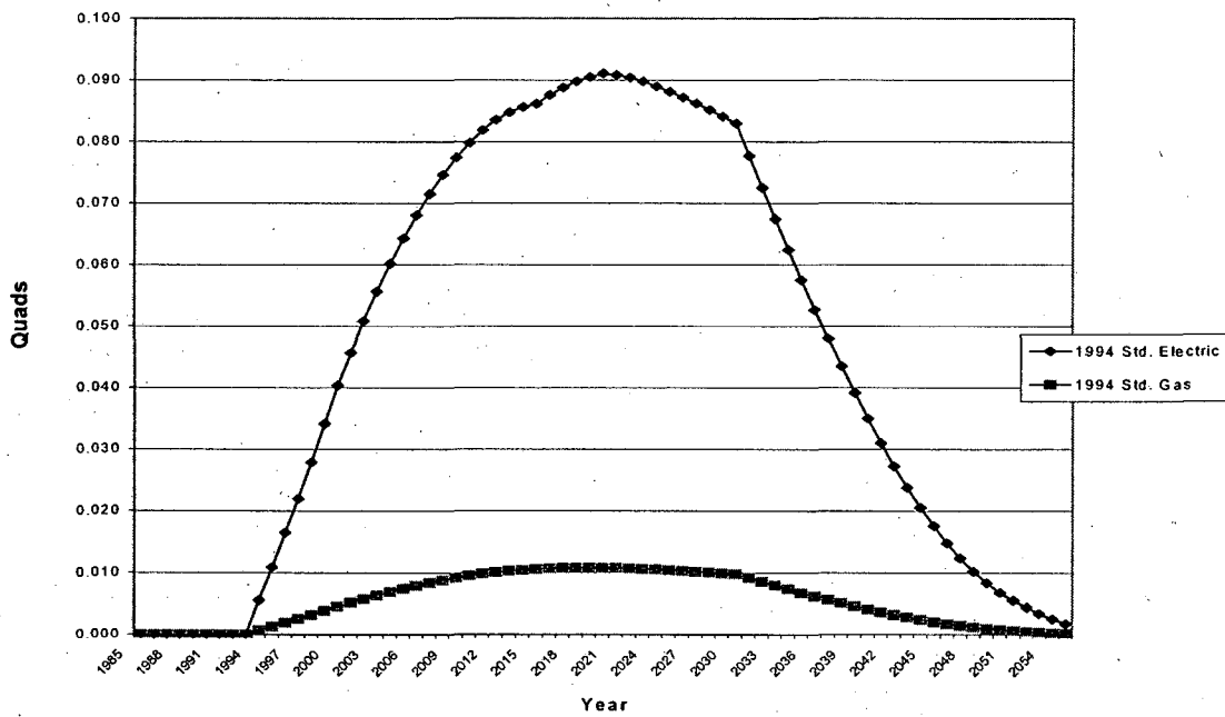
Figure 5.6 Clothes Dryer Standards Annual Primary Energy Savings, 1985-2055
