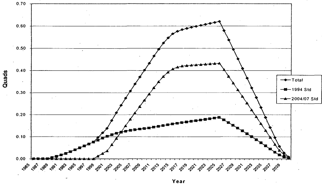
Figure 5.5 Clothes Washer Standards Annual Primary Energy Savings, 185-2050
