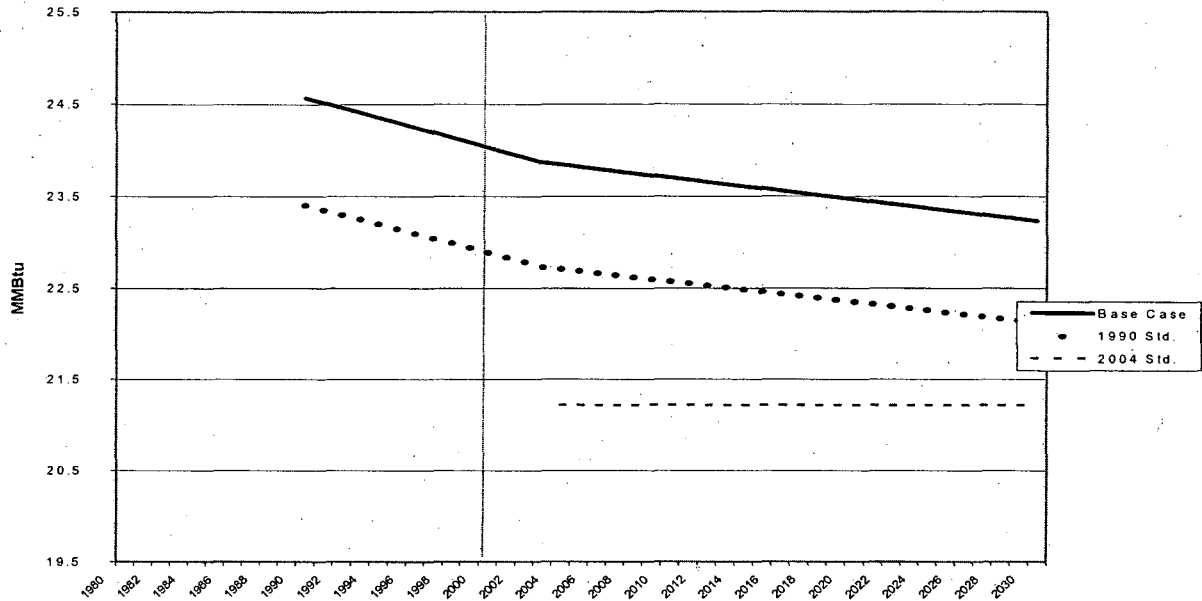
Figure 3.9 New Gas Water Heaters – Average Annual Energy Use, 1980-2030
