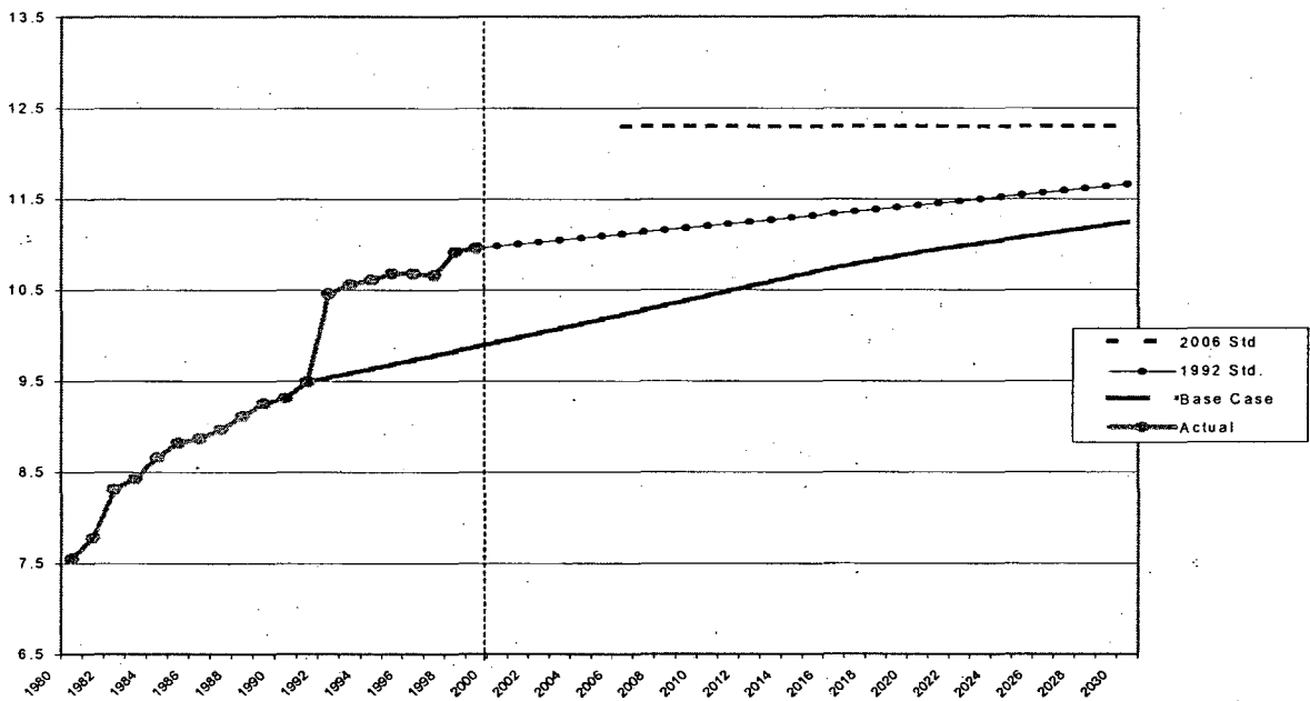
Figure 3.4 New Central Air Conditioners – Average SEER, 1980-2030
