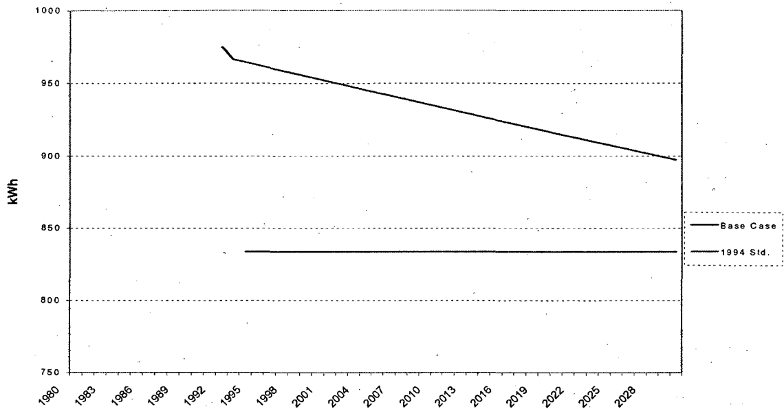
Figure 3.7 New Electric Clothes Dryers – Average Annual Electricity Use, 1980-2030
