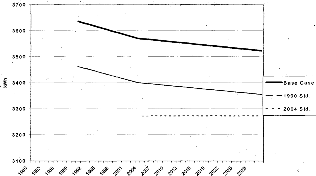
Figure 3.10 New Electric Water Heaters – Average Annual Energy Use, 1980-2030
