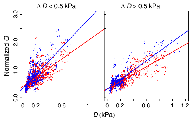
Fig. 5 Effects of clock regulation on plant water use. We compared the slopes of normalized sap flow ( Q ) in response to vapor pressure deficit ( D ) for eight Eucalyptus globulus trees between nights with little variation in D ( \Delta D < 0.5 kPa) and nights with large variation in D ( \Delta D > 0.5 kPa). We observed that the slope of this regression was always significantly higher ( t -test, P -value < 0.05 ) at predawn (●; 04:30–05:00 h) than at midnight (●; 00:00–00:30 h). This shows the effect of endogenous regulation over the whole-plant water flux, independent of the degree of environmental variation. Lines indicate the result of linear fitting.
