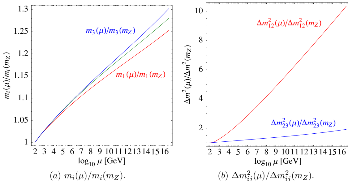
Figure 2: Example of the evolution of the mass eigenvalues and the \Delta m^2 s. We choose m_1(m_Z) = 0.1 eV, \delta(m_Z) = 50^\circ , \tan\beta = 50 and a SUSY breaking scale of 200 GeV, and best-fit values otherwise.
