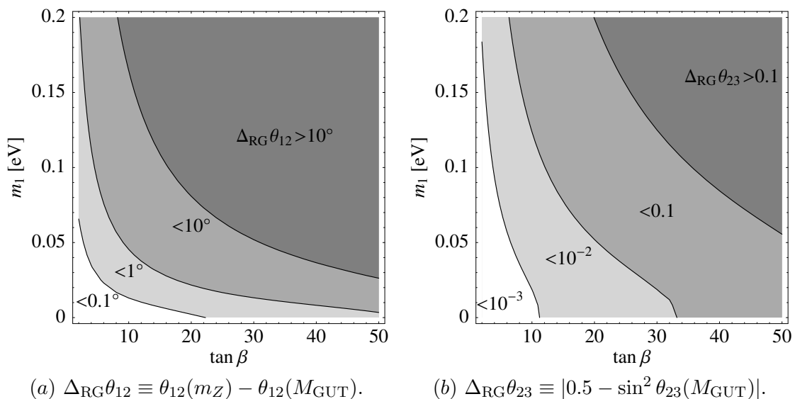
Figure 3: Radiative correction to (a) \theta_{12} and (b) \theta_{23} for \theta_{12} = 33^\circ , \theta_{13} = 10^\circ , \theta_{23} = 45^\circ and \delta = 90^\circ at \mu = m_Z as a function of \tan\beta and m_1 . These contours remain to a large extent unchanged when varying \theta_{13} in the allowed range and \delta arbitrarily.
