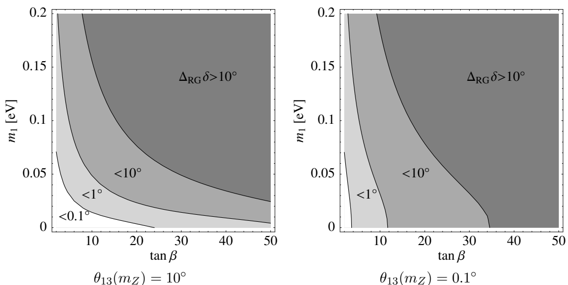
Figure 5: Radiative correction to \delta , defined as \Delta_{\text{RG}} \delta \equiv |\delta(m_Z) - \delta(M_{\text{GUT}})| for (a) \theta_{13}(m_Z) = 10^\circ and (b) \theta_{13}(m_Z) = 0.1^\circ as a function of \tan \beta and m_1 . We use \delta(m_Z) = 90^\circ .
