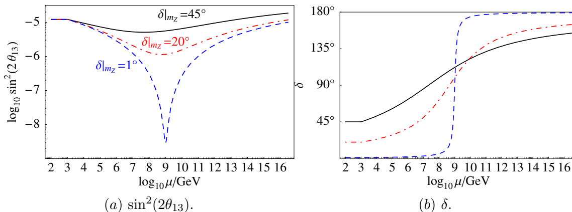
Figure 1: Evolution of (a) \sin^2(2\theta_{13}) and (b) \delta for small values of \theta_{13} . We use \tan\beta = 50 , \theta_{13} = 0.1^\circ , m_1 = 0.1 eV and best-fit values for all other parameters. The solid (black), dash-dotted (red) and dashed (blue) curve shows the evolution of (a) \theta_{13} and (b) \delta for \delta = 45^\circ , 20^\circ and 1^\circ at the electroweak scale, respectively. \theta_{13} cannot become 0 in any of the cases.
