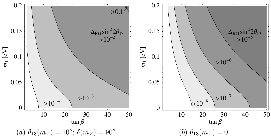
Figure 4: Radiative correction to \sin^2 2\theta_{13} , defined as \Delta_{\text{RG}} \sin^2 2\theta_{13} \equiv |\sin^2 2\theta_{13}(M_{\text{GUT}}) - \sin^2 2\theta_{13}(m_Z)| , as a function of \tan \beta and m_1 . We take \theta_{12}(m_Z) = 33^\circ and \theta_{23}(m_Z) = 45^\circ .
