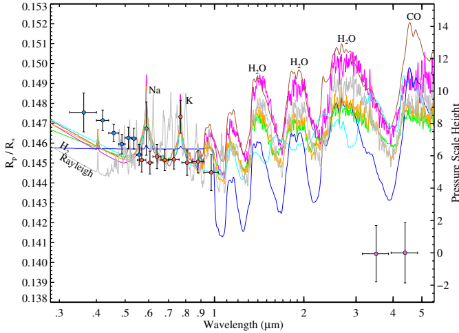
Figure 11. WASP-6b transmission spectrum compared to seven different cloud-free atmosphere models listed in Table 4, including Burrows-Dayside1200K-3×solar (brown), Burrows-Issth.1200K-high-CO (cyan), Burrows-Issth.1200K-ExtraAbsorber (blue), Fortney-Issth.1000K (green), Fortney-Issth.1500K-noTiO/VO (magenta), Fortney-PlanetAveraged1200K (orange) and Fortney-Issth.1500K-withTiO/VO (grey). All these models hardly reproduce the two Spitzer measurements. Prominent absorption features are labeled.
