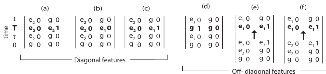
Fig. 1. Selected nonrephasing Liouville pathways contributing to beats in a 2D spectrum. States are written in a product basis of eigenstates, where subscripted letters denote electronic eigenstates and 0 or 1 is the vibrational occupation number at one of the two sites. Coherences observed over waiting time T are in bold.
