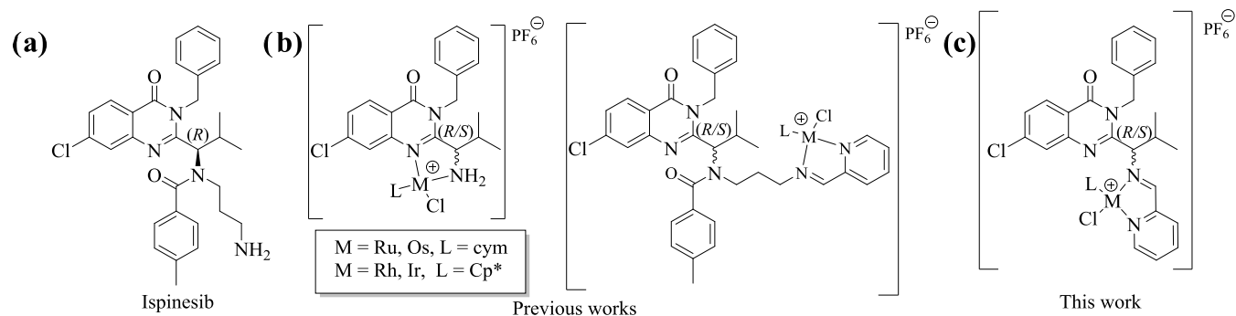
Figure 1. Structure of (a) ispinesib, (b) its quinazoline-derived Ru, Os, Rh, and Ir half-sandwich conjugates reported previously, 44,45 and (c) compounds studied herein.
