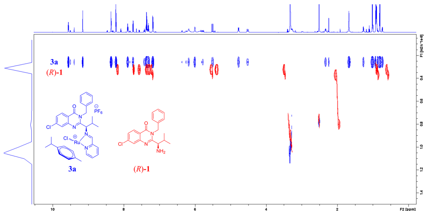
Figure 2. Overlapped 1 H DOSY spectra of 3a (blue) and (R)-1 (red) in DMSO- d 6 .
